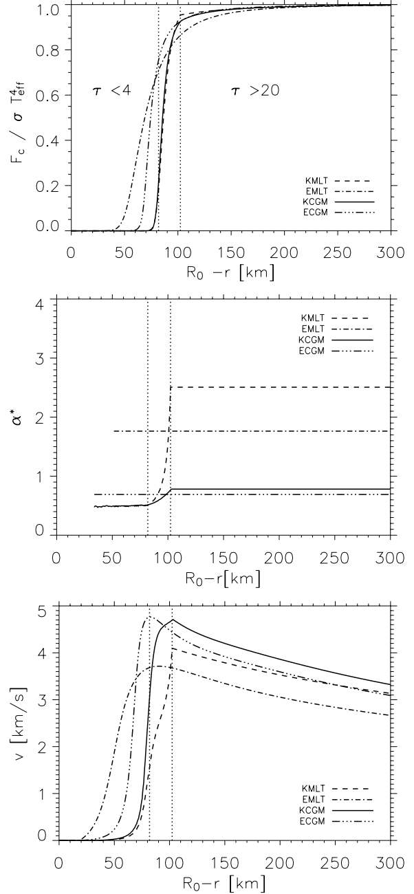
Fig. 3. Top: F_c is plotted versus R_\odot - r for the KMLT model (dashed curve), EMLT model (dot-dashed line), ECGM model (dot-dot-dot-dashed line), and KCGM model (solid line). As in Fig. 2, the dotted vertical lines delimit the transition region. Middle: same as the top panel for \alpha^* (see Sect. 3.2). Bottom: same as the top panel for the root mean square of the convective velocity, v .
