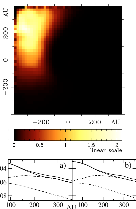
Fig. 18. Same as Fig. 15, but for a vertically thinner disc, described by Eq. (19). The total mass of the disc is the same as in the nominal case, but the asymmetries become prominent.
