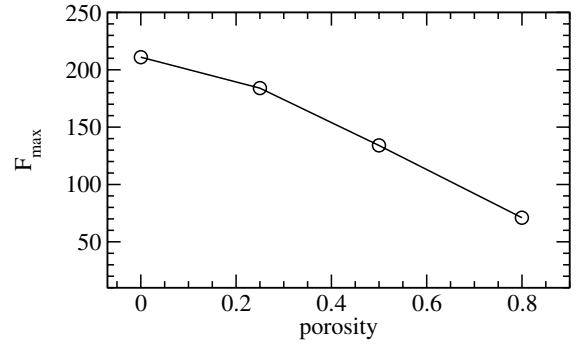
Fig. 11. Maximum amplification factor as a function of porosity for pure silicate grains. The value of the threshold energy, Q^* , is assumed to be the same as in the nominal case.
