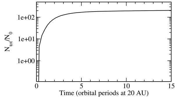
Fig. 4. Ratio of the total number of grains produced by the avalanche by the time t , N_{\text{tot}} , to the initial number of released planetesimal debris, N_0 .
