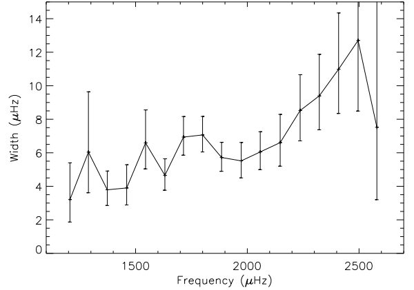
Fig. 4. Widths of the fitted modes, with 1\sigma error bars.
