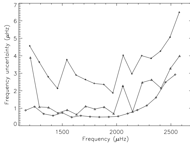
Fig. 9. Mean ( upper and lower ) 1\sigma error bars for the frequencies of l = 0 (triangles), l = 1 (diamonds) and l = 2 (crosses) modes, showing the decreasing precision on the frequencies from l = 1 to l = 2 modes.
