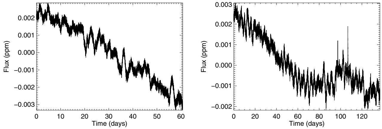
Fig. 7. Lightcurves of HD49933 for the 60-day long initial run ( left ) and the 137-day long run ( right ).
