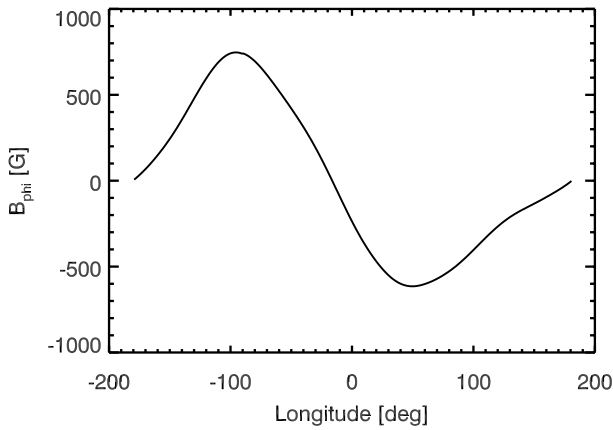
Fig. 4. Azimuthal component of the instability-generated magnetic field, at the peak of the instability ( \approx 10000 days, case A), measured at r/R_\odot = 0.7 , \theta = 75^\circ . Note that this non-axisymmetric field is dominated by the wavenumber m = 1 , which is the signature of the Pitts & Taylor instability.
