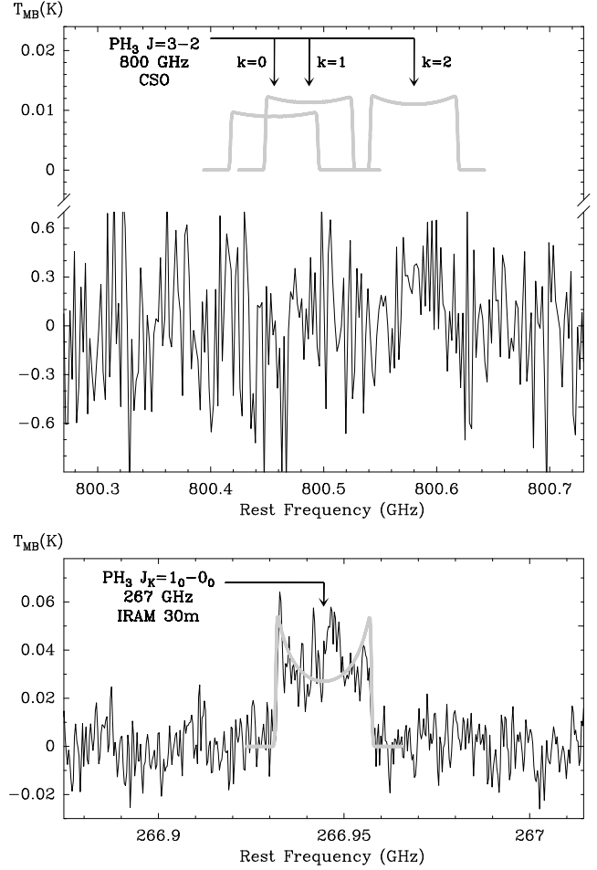
Fig. 2. The lower panel shows the PH 3 J_K = 1_0-0_0 line at 267 GHz as observed with the IRAM 30-m telescope, in which the fit to the SiS v = 4 J = 15-14 line has been subtracted. The upper panel shows the observation at 800 GHz with the CSO smoothed to a spectral resolution of 2 MHz. The thick grey lines in both panels correspond to the line profiles given by the LVG model.
