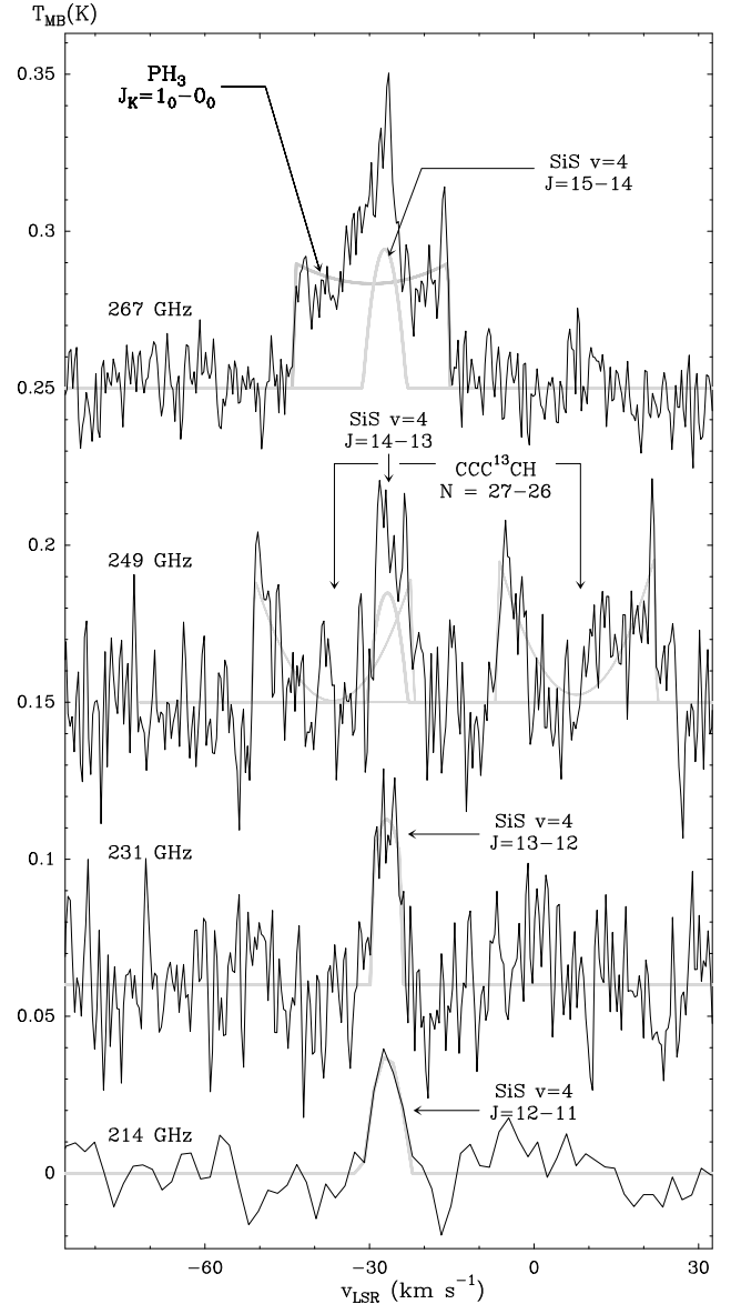
Fig. 1. Spectra of IRC +10216 observed with the IRAM 30-m telescope showing on top the J_K = 1_0-0_0 line of PH 3 blended with a narrower line assigned to the J = 15-14 line of SiS v = 4 . Shown below are the immediate lower rotational transitions of SiS v = 4 . Fits to the line profiles using the CLASS shell method are shown as thick grey lines.
