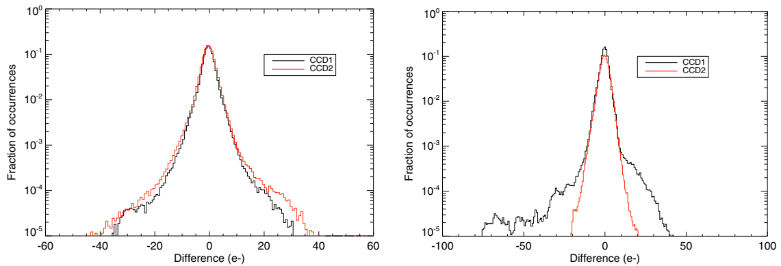
Fig. 10. On the left – the histogram of the differences for the triangle interpolation correction for the LRc01 using all windows. On the right – the same using only 32 s windows. Both use data corrected for bright pixels and smoothed over one hour. The abscissae ranges are not the same on these two plots due to extreme values that needed to be included.
