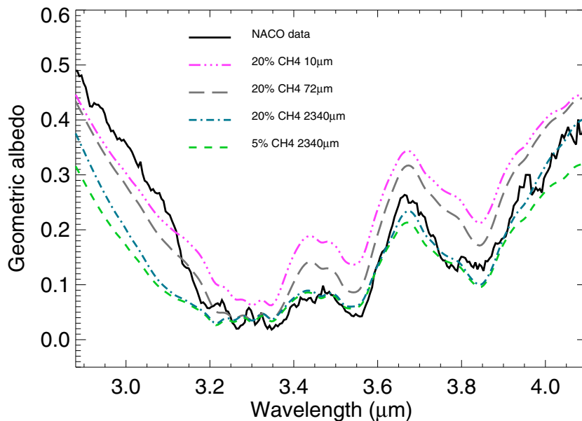
Fig. 12. Modeling results for different concentrations of pure methane and different grain sizes, compared with NACO L band spectrum of Pluto. By default, all the models assume 32% of pure \text{CH}_4 with 2340 \mu\text{m} grain size, 34% of \text{CH}_4 and \text{CO} ice diluted in \text{N}_2 with 95 \mu\text{m} grains, 6% of \text{CH}_2\text{CHCN} with 9 \mu\text{m} grains and 8% of titan tholin at 100 \mu\text{m} grains. Only the percentage of pure methane ice and its grain sizes are varied. The sensitivity of the L band spectrum to changes in the grain size of pure \text{CH}_4 is shown in the figure by some examples. (See the electronic version of the Journal for a color version of this figure.)
