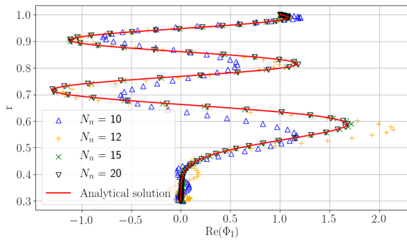
(a) Radial evolution of the eigenmode n = 5 (real part)
