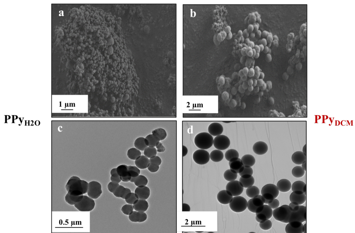
Figure 5- Morphological characterizations of radiosynthesized PPy polymers: SEM images of a) PPy H2O and b) PPy DCM polymers as well as TEM images of c) PPy H2O and d) PPy DCM polymers. PPy polymers were obtained after \gamma -irradiation at 72 kGy of an aqueous solution under N 2 O or a DCM solution under N 2 atmosphere. Initial concentration of Py monomers was 20 mM in all cases.
