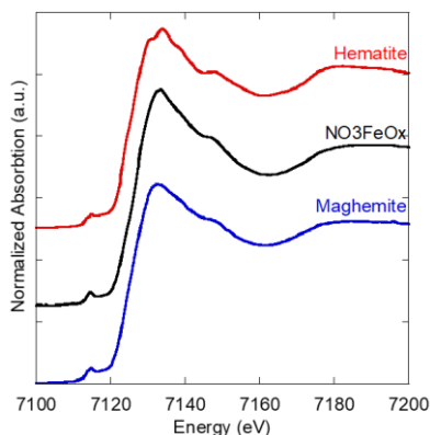
Fig. A1. Normalized Fe K-edge XANES spectra of NO 3 FeO x compared with the spectra of the maghemite and hematite references. It can be seen that the spectrum of NO 3 FeO x exhibits the same spectral features as the one of maghemite, whereas it is clearly different from the hematite one. This indicates the formation of maghemite rather than hematite in NO 3 FeO x . The spectra were measured in transmission mode on the SAMBA beamline at SOLEIL (Gif-sur-Yvette, France). They were conventionally normalized using the ATHENA software and energy calibrated after measurement. The acquisition was performed at room temperature in a continuous mode from 6900 eV to 8300 eV. No radiation damage was observed. The references were measured as pellets diluted in BN and NO 3 FeO x was placed between two pieces of kapton tape.
