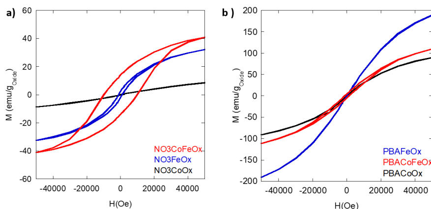
Fig. 6. Magnetic field dependence of the magnetization measured at 5 K of a) \text{NO}_3\text{CoOx} , \text{NO}_3\text{FeOx} , \text{NO}_3\text{CoFeOx} and b) \text{PBACoOx} , \text{PBAFeOx} , \text{PBACoFeOx} .
