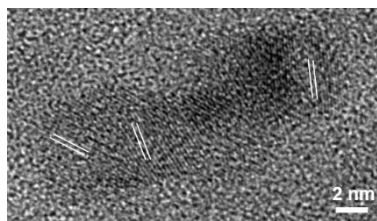
Fig. A2. HR-TEM image of NO 3 CoFeO x showing a polycrystalline nanorod.
