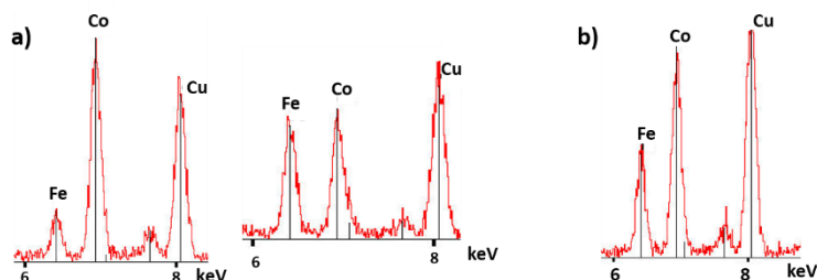
Fig. A3. Representative EDS spectra of a) NO 3 CoFeO x showing the strong variations of the Co/Fe ratio within the different regions of the nanoparticle assembly, and b) PBACoFeO x showing a Co/Fe ratio of 1.5.
