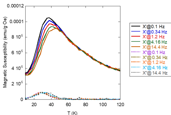
Fig. A4. Frequency-dependent AC magnetic measurements of NO 3 FeO x in the 10 -120 K temperature range.
