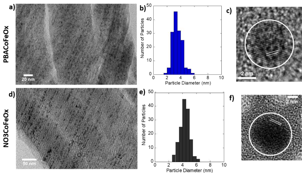
Fig. 4. Representative TEM images of a) PBACoFeOx and d) NO 3 CoFeOx ; particle diameter distributions for b) PBACoFeOx and e) NO 3 CoFeOx ; HR-TEM images of c) PBACoFeOx and f) NO 3 CoFeOx .
