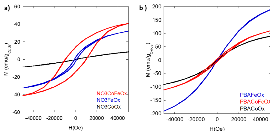
Fig. 6. Magnetic field dependence of the magnetization measured at 5 K of a) NO 3 CoOx , NO 3 FeOx , NO 3 CoFeOx and b) PBACoOx , PBAFeOx , PBACoFeOx .
