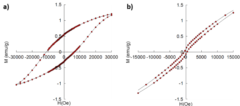
Fig. A6. Magnetization measured at 5 K after cooling from 300 K with an applied field of H = 30 kOe of a) NO 3 CoFeOx and b) PBACoFeOx.
