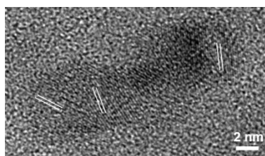
Fig. A2. HR-TEM image of \text{NO}_3\text{CoFeOx} showing a polycrystalline nanorod.
