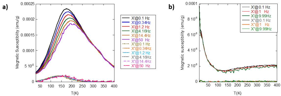
Fig. A5. In-phase ( \chi' ) and out-of-phase ( \chi'' ) components of the AC magnetic susceptibility as a function of temperature of a) NO 3 CoFeOx and b) PBACoFeOx.
