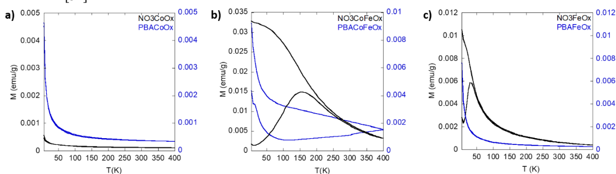
Fig. 5. ZFC-FC magnetization curves of the nanocomposites a) NO3CoOx and PBACoOx , b) NO3CoFeOx and PBACoFeOx , and c) NO3FeOx and PBAFeOx . The left y-axis corresponds to the NO 3 synthesis pathway and the right one to the PBA synthesis pathway.
