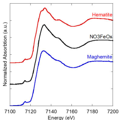
Fig. A1. Normalized Fe K-edge XANES spectra of \text{NO}_3\text{FeOx} compared with the spectra of the maghemite and hematite references. It can be seen that the spectrum of \text{NO}_3\text{FeOx} exhibits the same spectral features as the one of maghemite, whereas it is clearly different from the hematite one. This indicates the formation of maghemite rather than hematite in \text{NO}_3\text{FeOx} . The spectra were measured in transmission mode on the SAMBA beamline at SOLEIL (Gif-sur-Yvette, France). They were conventionally normalized using the ATHENA software and energy calibrated after measurement. The acquisition was performed at room temperature in a continuous mode from 6900 eV to 8300 eV. No radiation damage was observed. The references were measured as pellets diluted in BN and \text{NO}_3\text{FeOx} was placed between two pieces of kapton tape.
