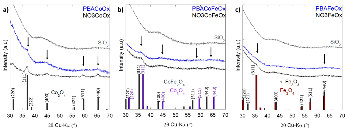
Fig.1. Powder X-ray diffraction patterns of the nanocomposites and the expected diffraction lines of the corresponding spinel oxides: a) NO3CoOx and PBACoOx compared to the diffraction lines of \text{Co}_3\text{O}_4 , NO3CoFeOx and PBACoFeOx compared to the diffraction line of \text{Co}_3\text{O}_4 and \text{CoFe}_2\text{O}_4 , and c) NO3FeOx and PBAFeOx compared to the diffraction lines of \gamma\text{-Fe}_2\text{O}_3 and \text{Fe}_3\text{O}_4 . The arrows indicate the position of the diffraction peaks. The diffraction pattern of the pure silica matrix is presented in each figure for comparison. The broad peak at 43^\circ 2\theta arises from the sample holder.
