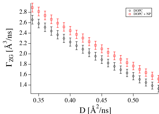
Fig. 7 Fit results for \Gamma_{ZG} assuming different translational diffusion coefficients using eq. (12). Regardless of the translational diffusion coefficient the same trend for the change of \Gamma_{ZG} upon NP addition is observed.
