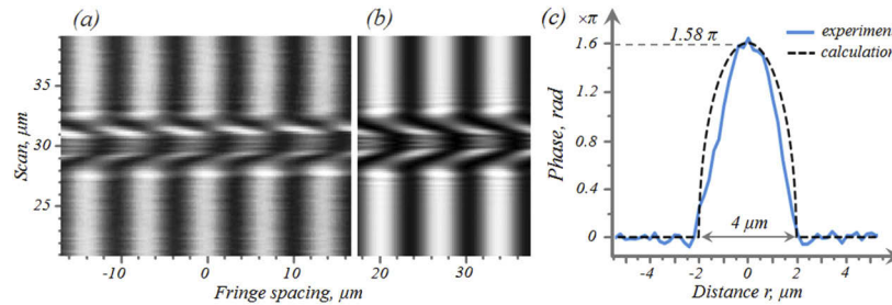
Fig. 5. The phase sensitivity study of the proposed imaging technique was carried out using a small tungsten fibre with a diameter of 4\ \mu\text{m} . (a) Experimental and (b) numerically simulated scan images. (c) Reconstruction of the phase profile of the tungsten fibre and the corresponding theoretical curve.
