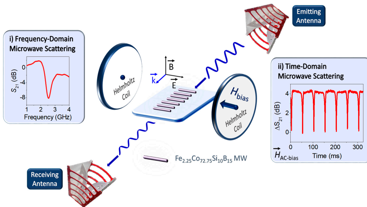
Figure 1. Schematic representation of the microwave scattering mechanism in transmission mode for sensing array platforms composed by \text{Fe}_{2.25}\text{Co}_{72.75}\text{Si}_{10}\text{B}_{15} (lengths of a few cm). Two Helmholtz coils apply axial magnetic fields to induce large changes in the magnetic state of the Co-based microwires (MWs) and then, giant magneto-impedance (GMI) effects arises. The S_{21} transmission coefficient is obtained in the (i) frequency and (ii) time domains.
