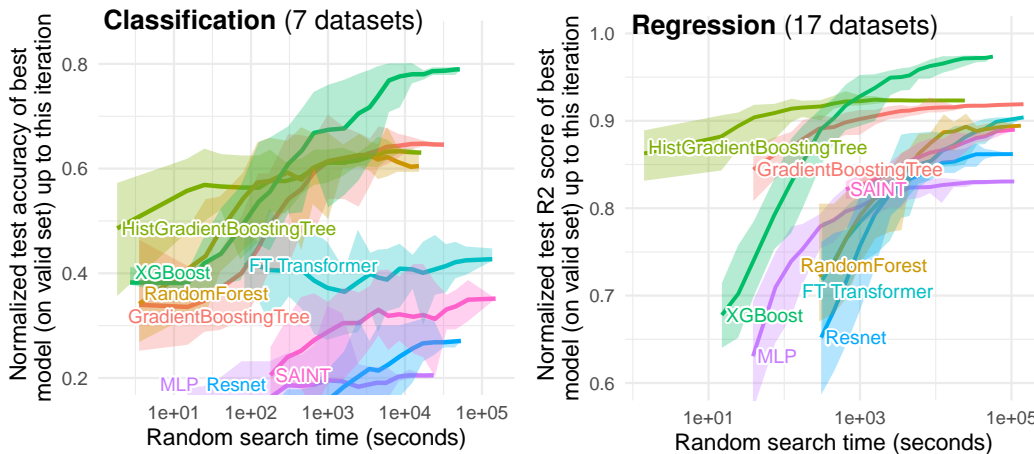
Figure 7: Time benchmark on medium-sized datasets, with both numerical and categorical features. The first random search iteration corresponds to default hyperparameters. Each value corresponds to the test score of the best model (on the validation set) after a specific time spent doing random search, averaged on 15 shuffles of the random search order. The ribbon corresponds to the minimum and maximum scores on these 15 shuffles.
