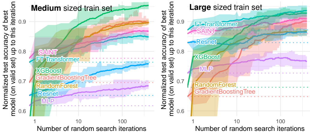
Figure 8: Comparison of accuracies on 5 classification tasks for different train set sizes, with only numerical features. Only datasets with more than 50,000 samples were kept, and the train set size was truncated to either 10,000 samples or 50,000 samples. Dotted lines correspond to the score of the default hyperparameters, which is also the first random search iteration. Each value corresponds to the test score of the best model (on the validation set) after a specific number of random search iterations, averaged on 15 shuffles of the random search order. The ribbon corresponds to the minimum and maximum scores on these 15 shuffles.
