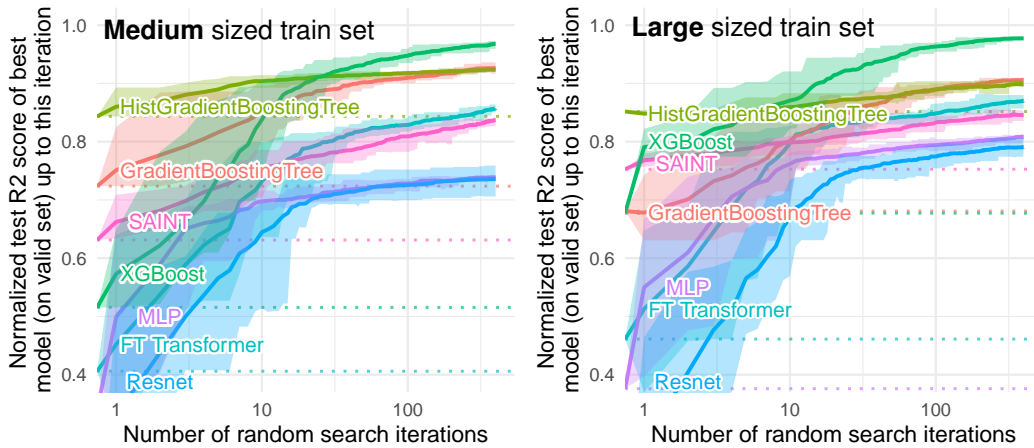
Figure 11: Comparison of R2 scores on 9 regression tasks for different train set sizes, with both numerical and categorical features. Only datasets with more than 50,000 samples were kept, and the train set size was truncated to either 10,000 samples or 50,000 samples. Dotted lines correspond to the score of the default hyperparameters, which is also the first random search iteration. Each value corresponds to the test score of the best model (on the validation set) after a specific number of random search iterations, averaged on 15 shuffles of the random search order. The ribbon corresponds to the minimum and maximum scores on these 15 shuffles.
