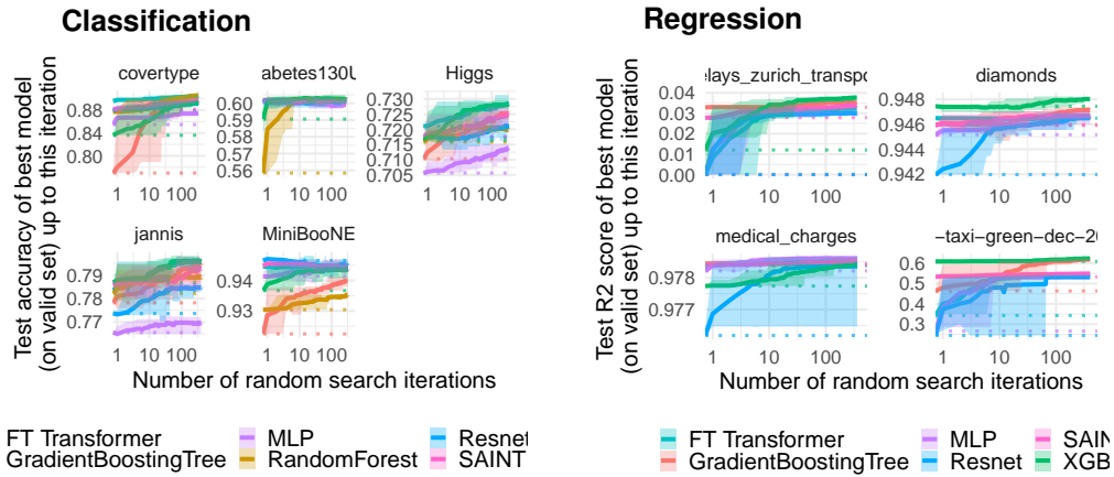
Figure 16: Unnormalized benchmark results for large scale datasets, for numerical features only.
