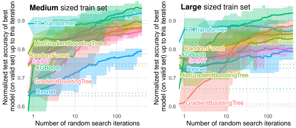
Figure 10: Comparison of accuracies on 3 classification tasks for different train set sizes, with both numerical and categorical features. Only datasets with more than 50,000 samples were kept, and the train set size was truncated to either 10,000 samples or 50,000 samples. Dotted lines correspond to the score of the default hyperparameters, which is also the first random search iteration. Each value corresponds to the test score of the best model (on the validation set) after a specific number of random search iterations, averaged on 15 shuffles of the random search order. The ribbon corresponds to the minimum and maximum scores on these 15 shuffles.
