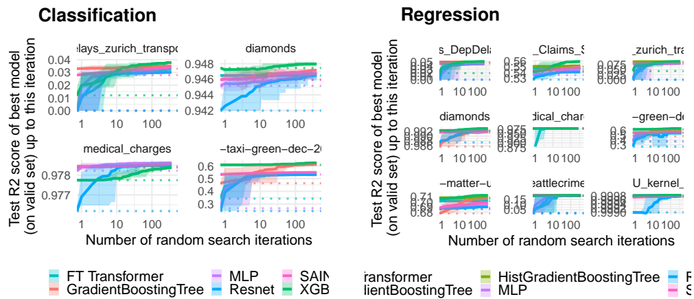
Figure 17: Unnormalized benchmark results for large-scale datasets, for both numerical and categorical features.
