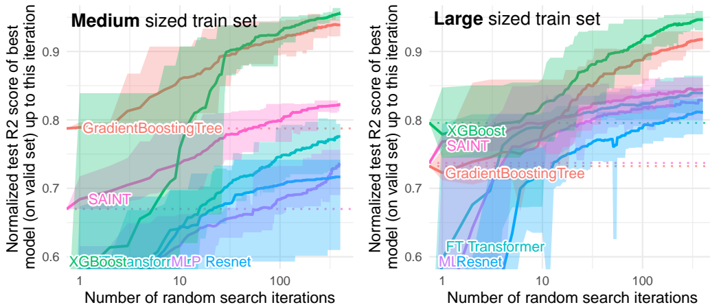
Figure 9: Comparison of R2 scores on 4 regression tasks for different train set sizes, with only numerical features. Only datasets with more than 50,000 samples were kept, and the train set size was truncated to either 10,000 samples or 50,000 samples. Dotted lines correspond to the score of the default hyperparameters, which is also the first random search iteration. Each value corresponds to the test score of the best model (on the validation set) after a specific number of random search iterations, averaged on 15 shuffles of the random search order. The ribbon corresponds to the minimum and maximum scores on these 15 shuffles.
