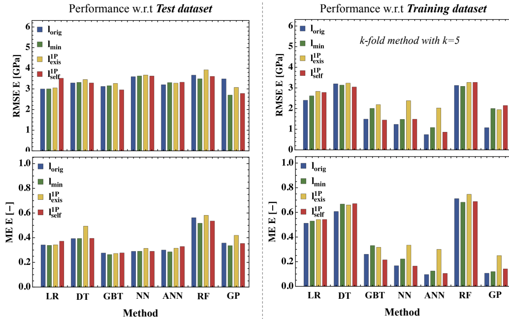
Figure 9: RMSE and ME computed for the test dataset (left) and using a cross-validation approach ( k = 5 folds) on the training dataset (right) for various ML methods using only the original training dataset l_{orig} , or extended training datasets l_{min} , l_{exis}^{1P} , or l_{self}^{1P} . New data is generated with SC1S_{Ellip} .
