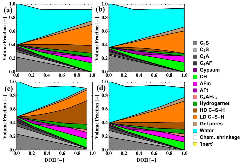
Figure 11: Volume fraction of phases for three commercial cements studied in refs. (a) (Honorio, Bary, and Benboudjema 2016; Honorio, Bary, and Benboudjema 2018; Honorio, Bary, Benboudjema, and Poyet 2016), (b) (Wyrzykowski et al. 2017) and (c) (Termkhajornkit et al. 2012), with w/c = 0.5 , as a function of the degree of hydration (DOH). The variations on C_3A content lead to significant differences in the emergence of various Al-bearing phases.
