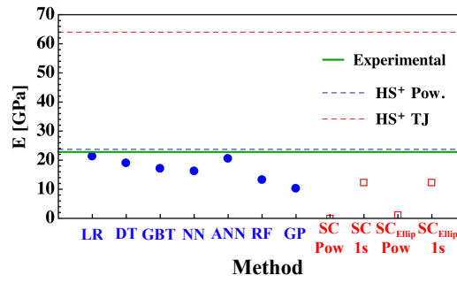
Figure 5: Prediction of the Young modulus E to reproduce the experimental observation by Constantinides and Ulm (Constantinides et al. 2004) (solid green line): results from ML (full blue dots) and MB (red empty dots) methods. Hashin-Shtrikman upper bounds using Powers and TJ model (dashed lines) are shown for reference.
