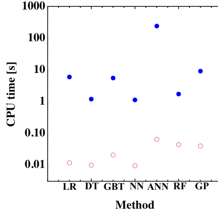
Figure 10: CPU time associated with the creation of the predictor functions based on the training dataset (full blue dots), and with one prediction using the already created predictor functions (empty red dots) for the various ML methods.
