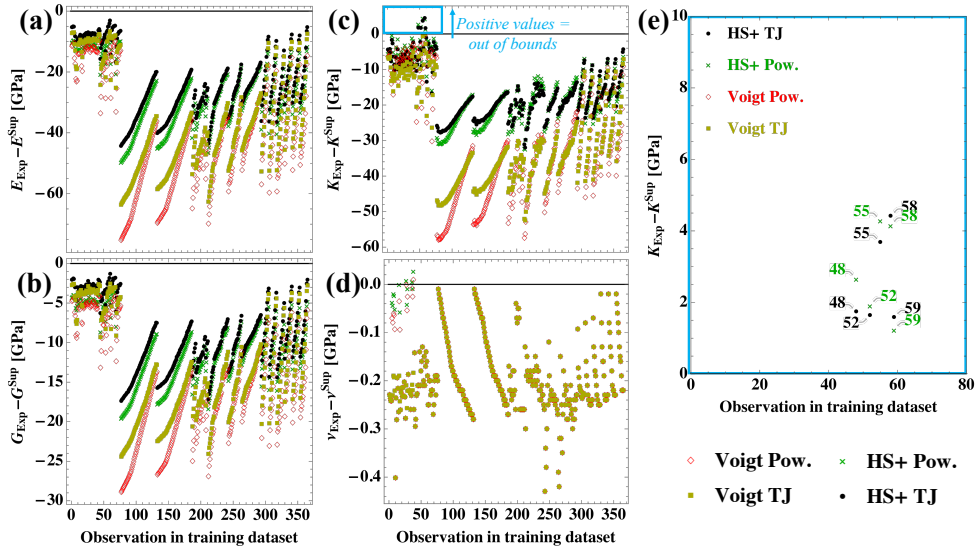
Figure 13: Difference between the experimental values in the dataset (subscript Exp ) and the Voigt and Hashin-Shtrikman upper bounds (superscript sup ) of (a) E , (b) G , (c) K and (d) \nu . (e) Identification numbers of the few experimental observations of K exceeding the theoretical upper bounds.
