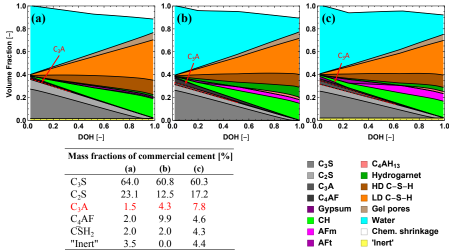
Figure 11: Volume fraction of phases for three commercial cements studied in refs. (a) (Honorio, Bary, and Benboudjema 2016; Honorio, Bary, and Benboudjema 2018; Honorio, Bary, Benboudjema, and Poyet 2016), (b) (Wyrzykowski et al. 2017) and (c) (Termkhajornkit et al. 2012), with w/c = 0.5 , as a function of the degree of hydration (DOH). The variations on C_3A content lead to significant differences in the emergence of various Al-bearing phases.
