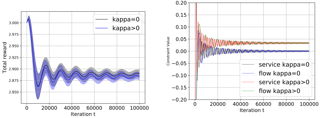
Figure 1: Learning Process of the proposed algorithm for linear objective and constraint value with \kappa = 0 and \kappa > 0 . The total reward is the objective in (31) with c = 0 and the constraint value is the L.H.S. of the constraint in (31).
