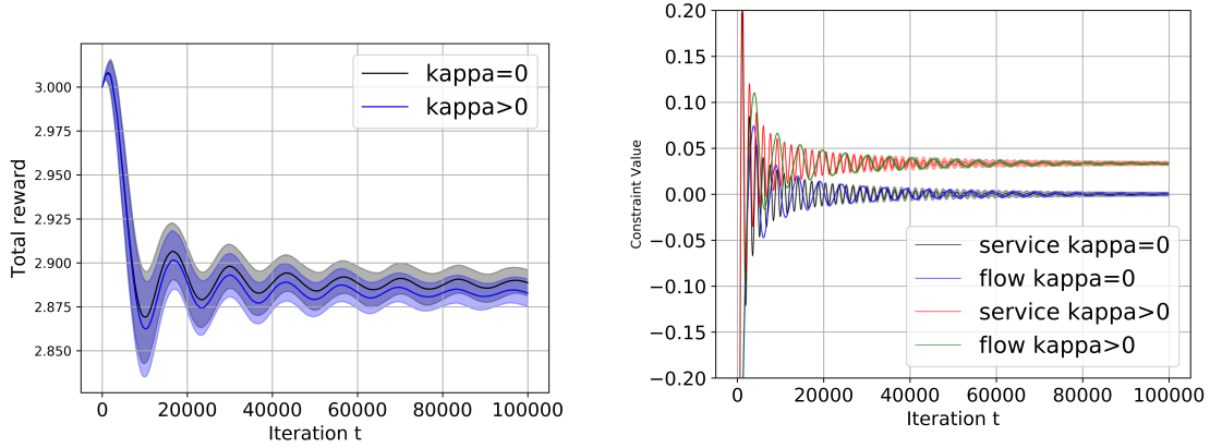
Figure 2: Learning Process of the proposed algorithm for concave objective and constraint value with \kappa = 0 and \kappa > 0 . The total reward is the objective in (31) with c = 1 and the constraint value is the L.H.S. of the constraint in (31).
