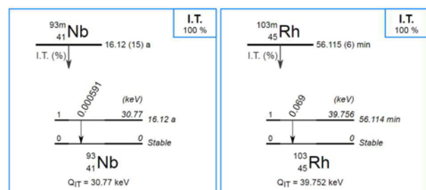
Fig. 1. Decay scheme of ^{93m}\text{Nb} (left) and ^{103m}\text{Rh} (right) [5]
