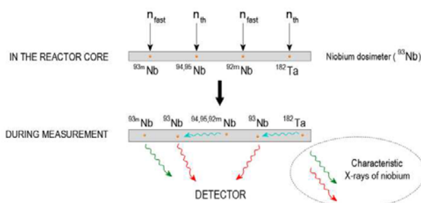
Fig. 6. Scheme of the self-fluorescence in a niobium dosimeter
