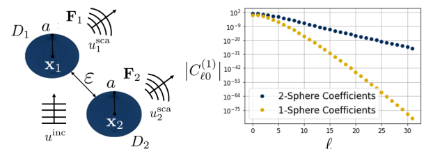
Figure 1: (Left) Sketch of the problem and notations. (Right) Plot of the expansion coefficients (C_{\ell 0}^{(1)})_{\ell \in \llbracket 0, 32 \rrbracket} in (5) for k = 7.33 , a = 0.16 , \mathbf{x}_1 = (0, 0, 0) , \mathbf{x}_2 = (0, 0, 2a + 1) ( \varepsilon = 1 ). The blue curve represents obtained (C_{\ell 0}^{(1)})_{\ell} when approximating (4) using Gaussian Product Quadrature rule (GPQ), the yellow curve refers to (C_{\ell 0}^{(1)})_{\ell} obtained analytically when there is only D_1 .
