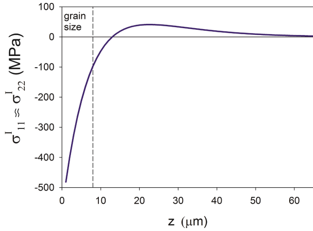
Fig. 16. The in-depth dependence of grain interaction, described by the stresses \sigma_{11}^I \approx \sigma_{22}^I in function of the real depth z , for tunable free-surface model. The assumed stress evolution function is given by Eq. (22). The dashed line marks the mean grain size of 8 \mu\text{m} .
