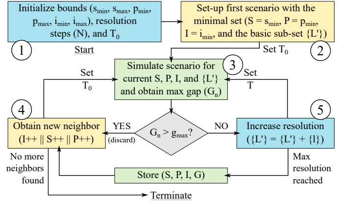
Fig. 4: Complexity-progressive gradient descent algorithm for sparse DtS-IoT constellation design [17].
