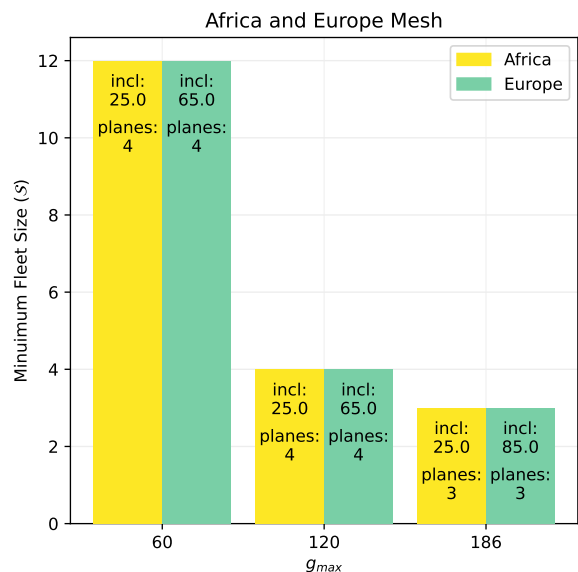
Fig. 12: Minimum Constellation Sizes for Africa and Europe ( g_{max} = \{60, 120, 186\} minutes, swath= 127.1^\circ ).
