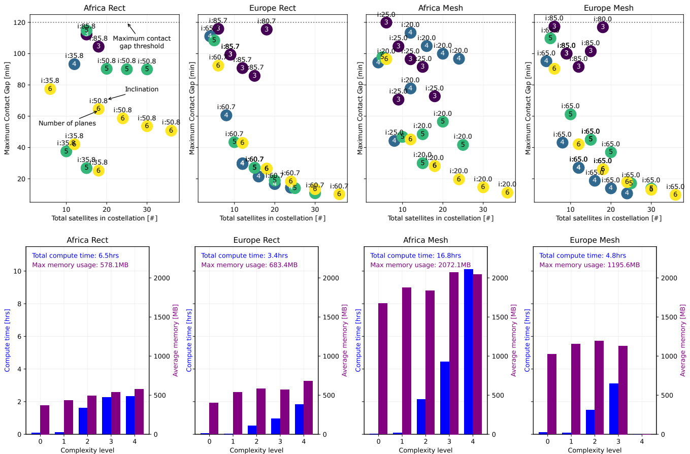
Fig. 8: Algorithm Performance Metrics for Europe and Africa ( g_{max} = 120 min) using Rectangular and Hexagonal Mesh Bounds for \{\mathcal{L}\} (top). Algorithm Resource Consumption Metrics in terms of compute time and memory consumption for the above corresponding cases (bottom).
