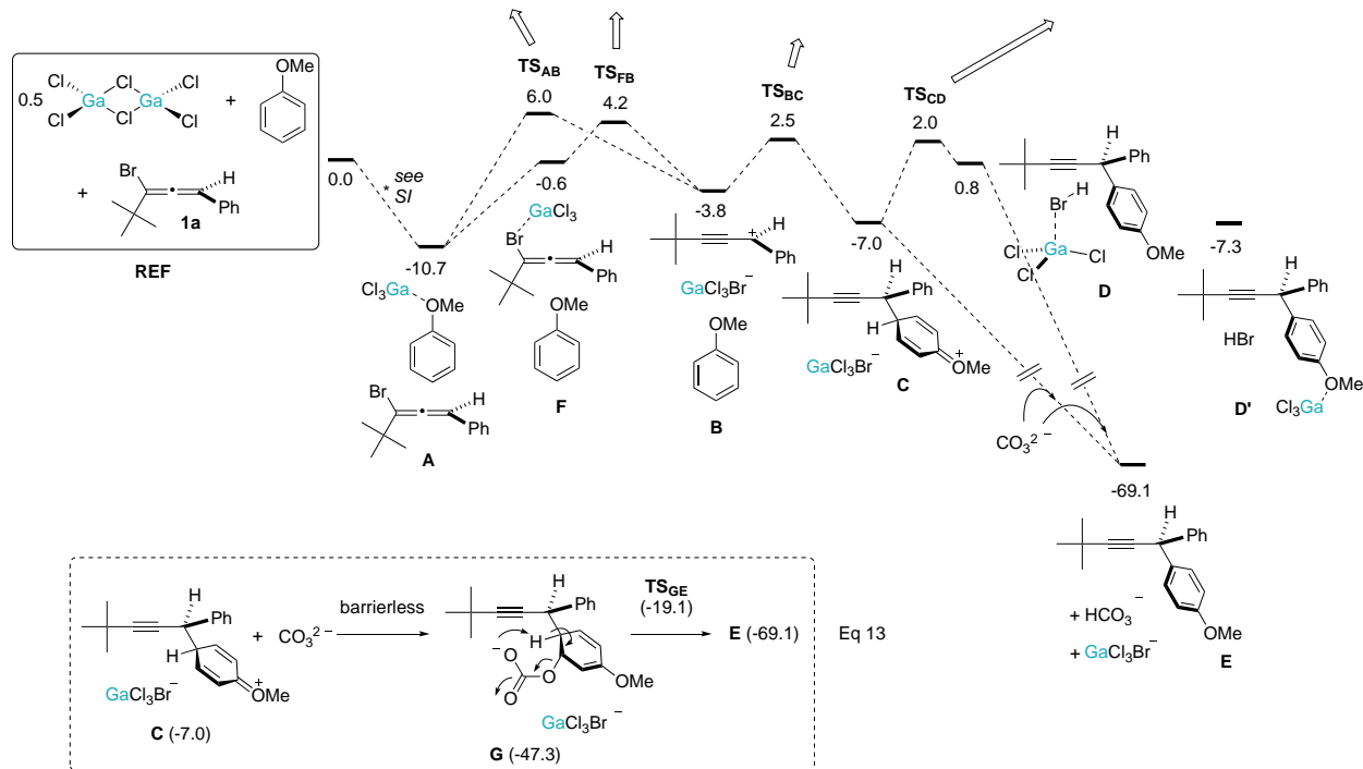
Scheme 8. Free Energy Profile ( \Delta G_{298} , kcal/mol) of the Gallium-Catalyzed C–H Propargylation of Anisole with Bromoallene 1a (* see the Supporting Information for the dissociation of \text{Ga}_2\text{Cl}_6 , Figure S25).
