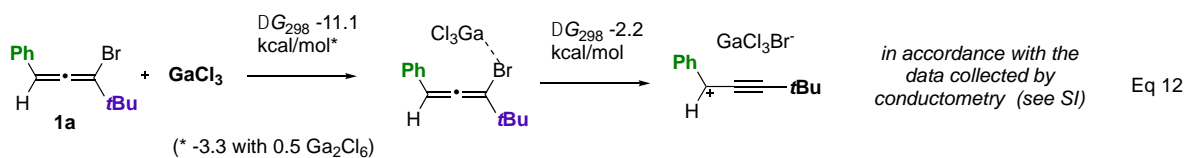
Scheme 6. Mechanistic Experiments.
