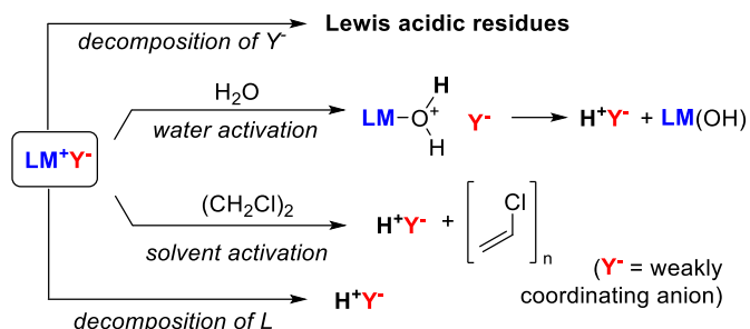
Scheme 1. Possible Decomposition Pathways Leading to the Real Active Species.
