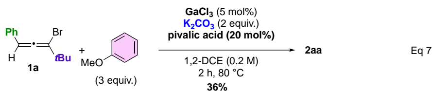
Scheme 4. Control Experiments.
