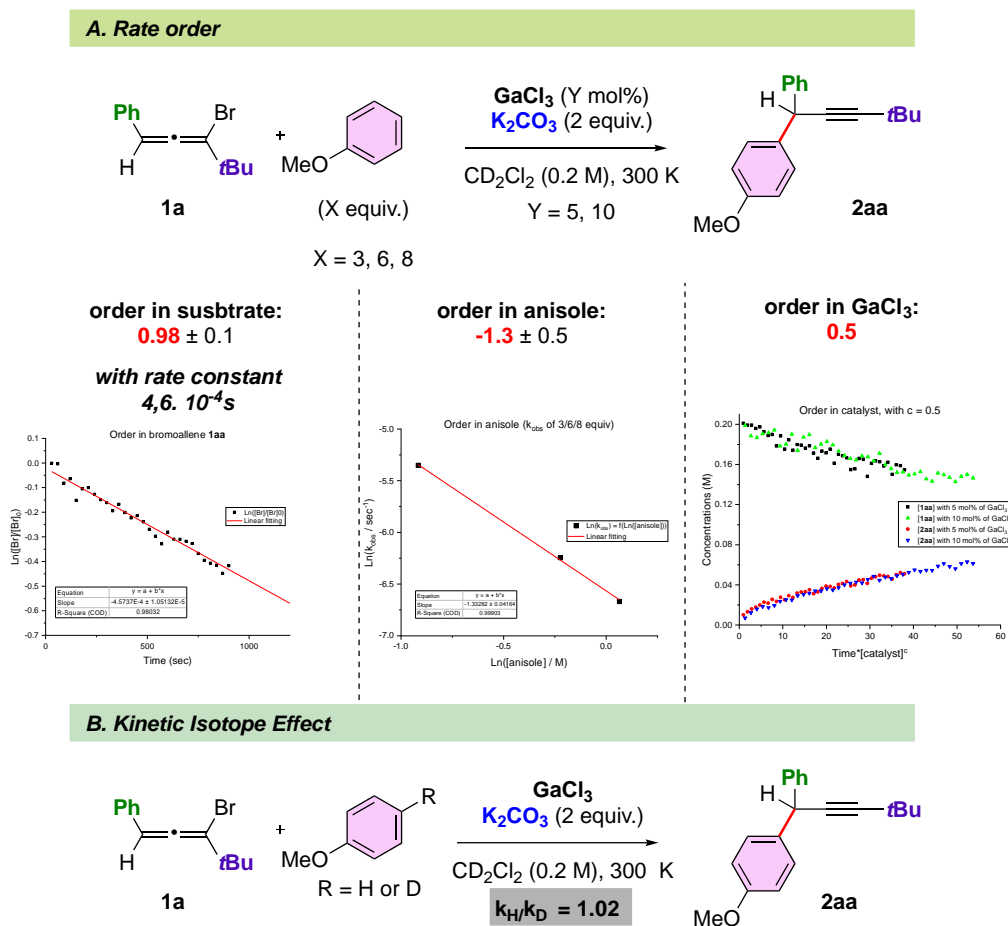
Scheme 7. Kinetic Investigations of the Gallium-Catalyzed C–H Propargylation of Arenes Based on the Consumption of the Substrate using three independent methods relying on “degeneration of order”, “initial rate” and “normalized time scale method”.
