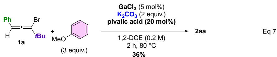
Scheme 4. Control Experiments.
