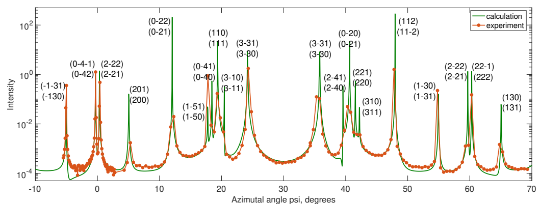
Figure 4. Azimuthal dependence of intensity of three-wave reflections at the photon energy E = 4.5 keV in the geometry of the forbidden reflection (001) in the right \alpha -quartz.
