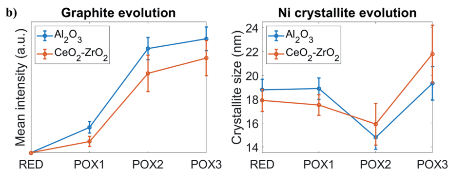
Fig. 10 (Panel a) Spatial distribution of ZrO 2 , graphite and metallic Ni crystallite size obtained through Rietveld analysis performed on XRD-CT data collected for various conditions: reduction, POX1, POX2 and POX3 from the middle of catalyst bed (middle of 3D-XRD-CT data volume). The observed reduction of Ni crystallite size is in fact a result of carbon intercalation. (Panel b) Evolution of graphite concentration and Ni crystallite size at the catalyst particles where CeO 2 –ZrO 2 (shell) and Al 2 O 3 (core) are primarily present.
