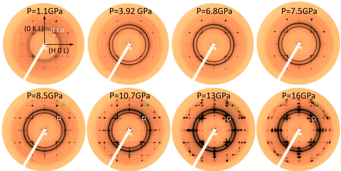
Figure 2. Diffraction patterns as a function of pressure. We observe a well-defined tetragonal structure at low pressures, with diffuse stripes that indicate a fluctuating 1D linear oxygen ordering along the two tetragonal axes [7]. Above 8 GPa, we observe the appearance of superstructure spots (indicated by light green and white circles). They become more intense and diffuse at very high pressures.
