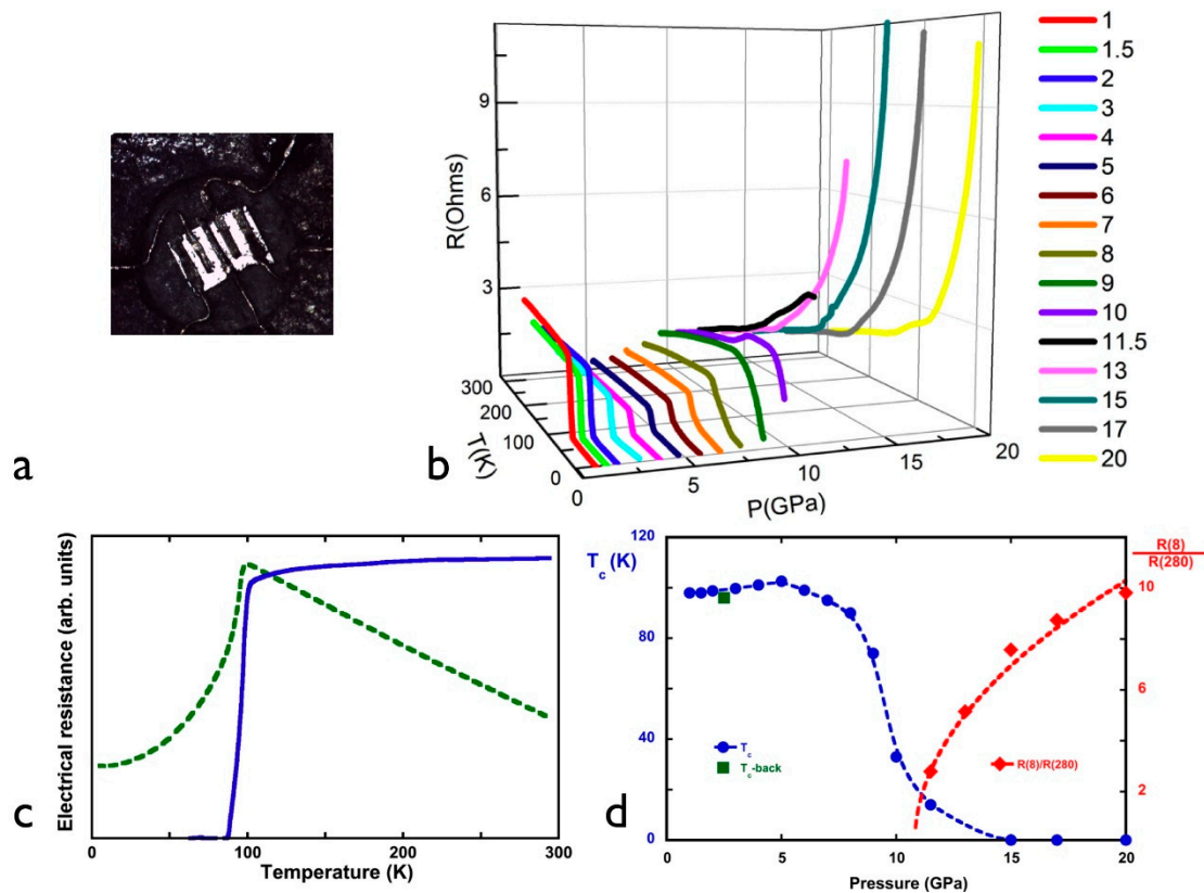
Figure 1. (a) Single crystal of Hg-1201 mounted in the pressure cell; (b) electrical resistance of the Hg-1201 single crystal as a function of pressure and temperature. The evolution from a metallic and superconducting behavior to an insulating (indicating charge-order) and non-superconducting one at high pressures is evident; (c) comparison of the resistivities at 4 GPa on compression and decompression. The superconducting behavior is recovered although the decompressed sample does not show a clear metallic behavior; and (d) in blue circles, we show the evolution of T_c with pressure. It increases up to about 5 GPa and further decreases to attain zero at 15 GPa. The red diamonds correspond to the ratio R(8K)/R(280) , a way of showing the increase in the charge ordering with pressure. The dashed red curve is a mean-field power law fit.
