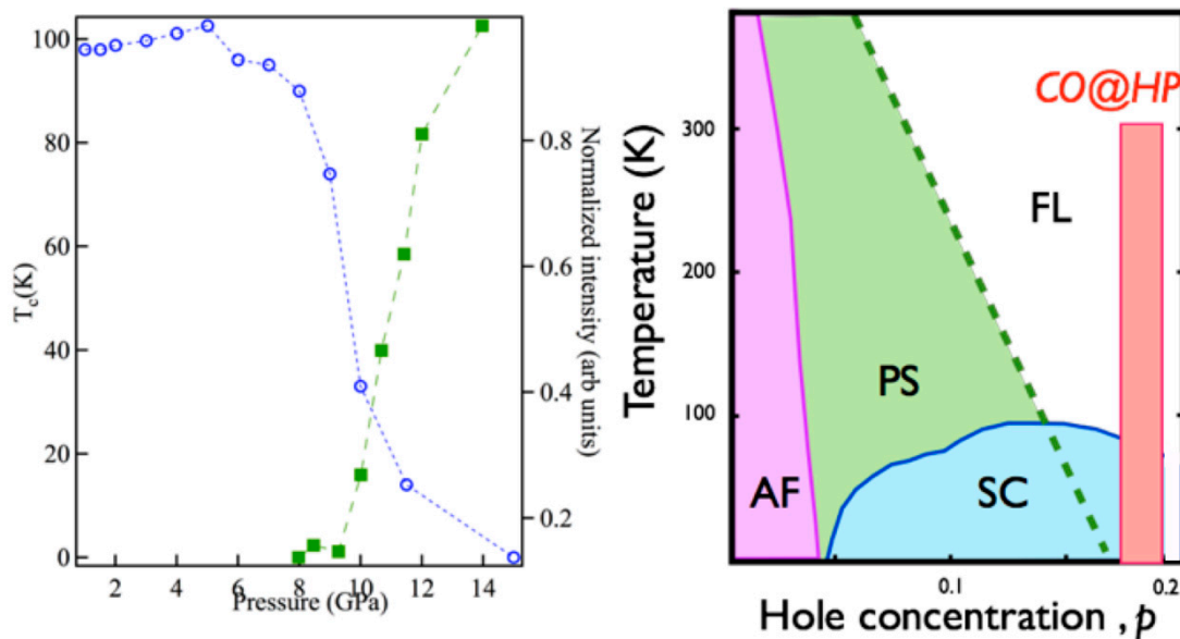
Figure 3. (left panel) Normalized intensity of the superstructure spots as a function of pressure compared to the evolution of T_c ; and (right panel) phase diagram of mercury cuprates showing where our results are situated as a function of doping.
