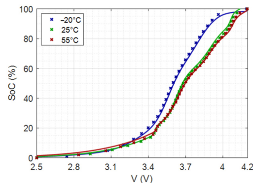
Figure 10. Estimation of the SoC at different voltages and temperatures using the proposed SoC = f(V, T) model. Crosses represent experimental data while lines are the combined models.
