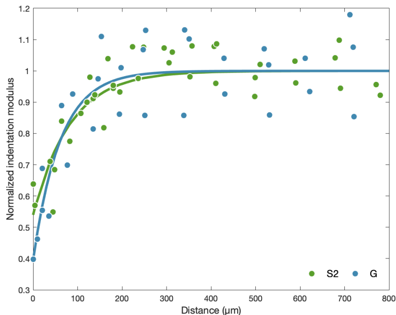
Figure 7: Normalized indentation modulus of the S_2 and G-layers from Fig. 6 as a function of the distance from the cell where the layer concerned first appeared. The solid line corresponds to the mean value.
