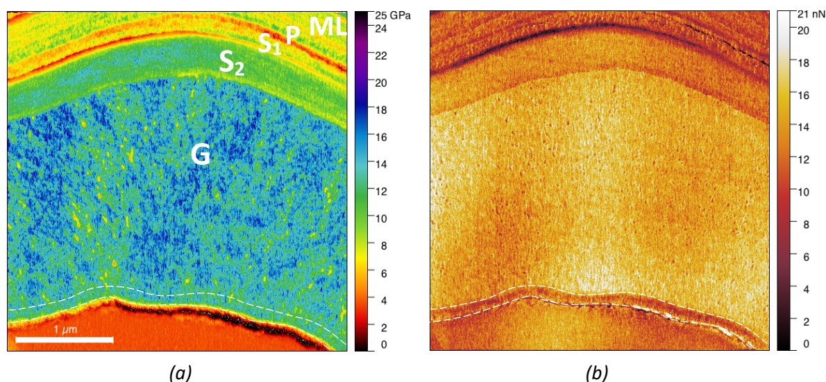
Figure 4: a) Close-up of the indentation map of a cell taken at a distance of 740 \mu\text{m} from the cambium corresponding to the white box in Fig. 2b, with the associated adhesion map (b), highlights a sub-G-layer with lower adhesion force close to the lumen.
