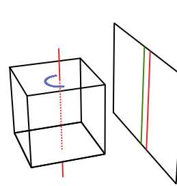
Fig. 6. A single-axis parallel beam acquisition with a custom center of rotation. An object, whose changing position during rotation is indicated in blue, is rotated around a non-standard axis of rotation (in red). The center of the detector is indicated in green.
