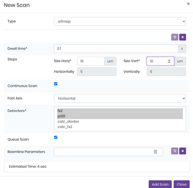
Figure 3 An example new scan dialogue where the user can select the type of action to execute against a particular ROI or POI. In this case an ROI is selected and the user can execute a 2D \mu XRF map. The form is automatically generated from the relevant actor's schema and parameter values are validated both in the client and on the server.
