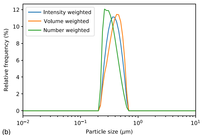
Fig. 7. Results from dynamic light scattering on supernatant from sedimentation test on Utby clay from 6-m depth. Results from unfiltered and filtered ( 2.5\text{-}\mu\text{m} filter) diluted supernatant samples are presented.
