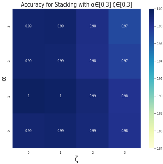
Figure. 17: Accuracy of Stack classifier for \alpha \in [0, 3] and \zeta \in [0, 3] with formula 1
