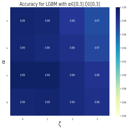
Figure. 11: Accuracy of LGBM classifier for \alpha \in [0, 3] and \zeta \in [0, 3] with formula 1
