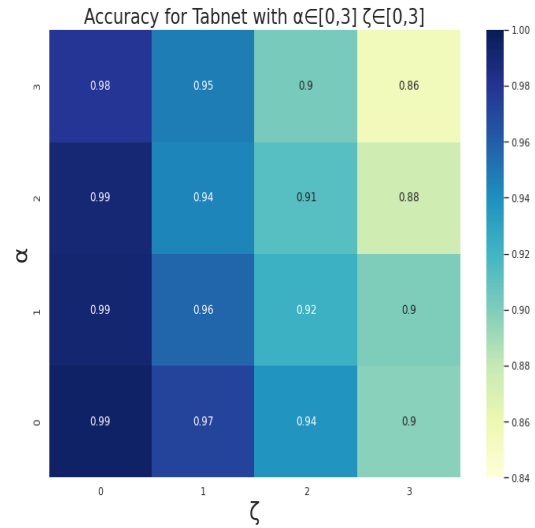
Figure. 14: Accuracy of TabNet classifier for \alpha \in [0, 3] and \zeta \in [0, 3] with formula 2
