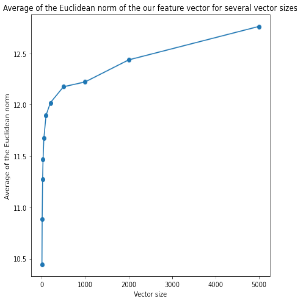
Figure. 4: Average of the Euclidean norm of the our feature vector for several vector sizes
