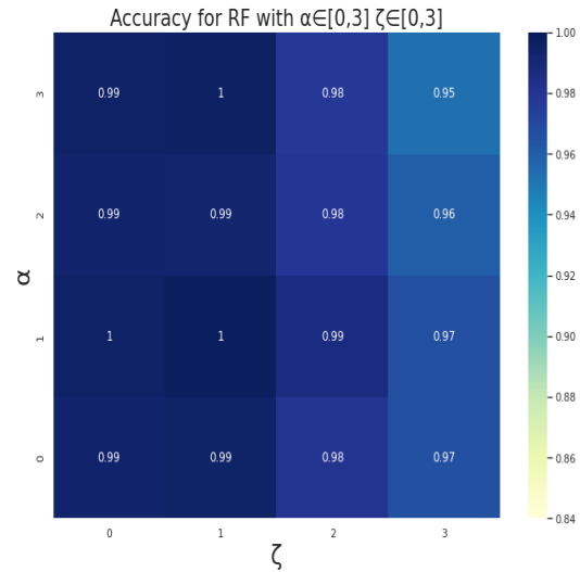
Figure 7: Accuracy of RF classifier for \alpha \in [0, 3] and \zeta \in [0, 3] with formula 1
