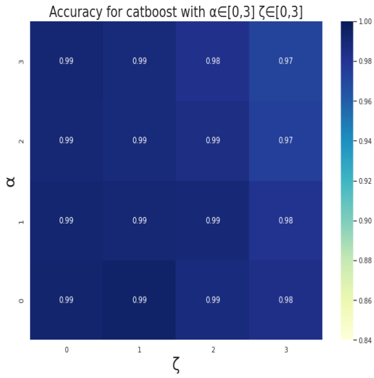
Figure. 10: Accuracy of catboost classifier for \alpha \in [0, 3] and \zeta \in [0, 3] with formula 2
