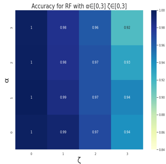
Figure 8: Accuracy of RF classifier for \alpha \in [0, 3] and \zeta \in [0, 3] with formula 2
