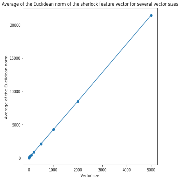
Figure. 3: Average of the Euclidean norm of the sherlock feature vector for several vector sizes
