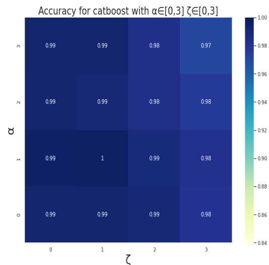
Figure 9: Accuracy of catboost classifier for \alpha \in [0, 3] and \zeta \in [0, 3] with formula 1
