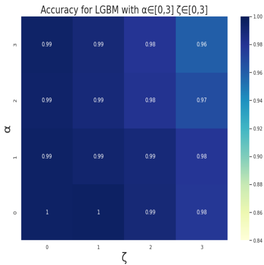
Figure. 12: Accuracy of LGBM classifier for \alpha \in [0, 3] and \zeta \in [0, 3] with formula 2
