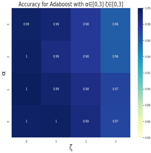
Figure. 16: Accuracy of Adaboost classifier for \alpha \in [0, 3] and \zeta \in [0, 3] with formula 2
