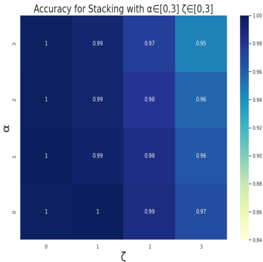
Figure. 18: Accuracy of Stack classifier for \alpha \in [0, 3] and \zeta \in [0, 3] with formula 2
