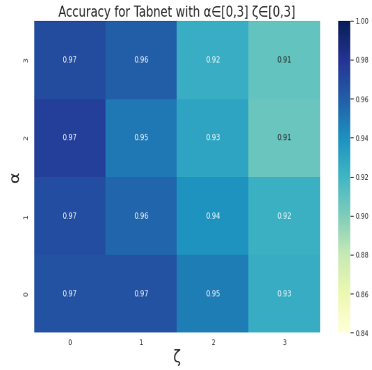
Figure. 13: Accuracy of TabNet classifier for \alpha \in [0, 3] and \zeta \in [0, 3] with formula 1
