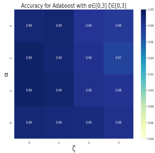
Figure. 15: Accuracy of Adaboost classifier for \alpha \in [0, 3] and \zeta \in [0, 3] with formula 1
