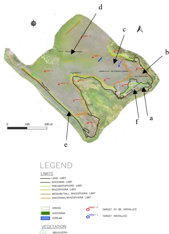
Figure 3. Topographic plan on an orthophoto. The red dots represent the targets that will be used for aerial photogrammetry. Arrows indicate (a) the tannin area, (b) the Avicennia Stylosa , (c) the medium Rhizophora , (d) the tall Rhizophora , (e) the pneumatophores and (f) the seagrass beds.
