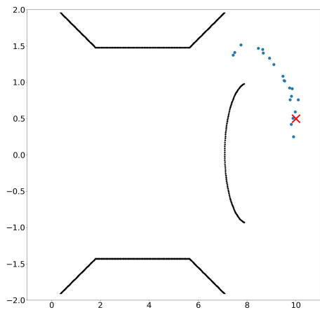
Figure 3.6: Time evolution of a swarm of N = 50 drones starting on the left of the simulation domain and converging towards a target (red point), by avoiding obstacles on their way.
