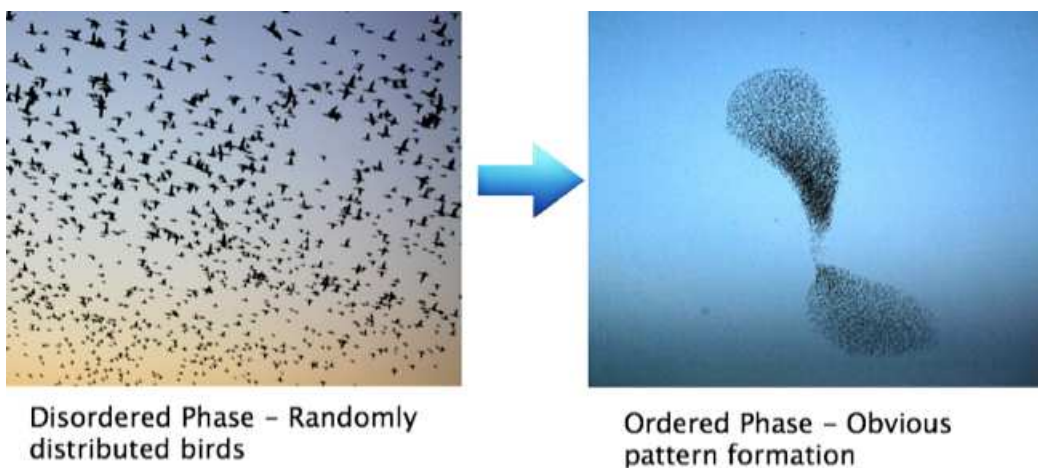
Figure 3.5: Examples of phase-transition in a bird swarm [30].
