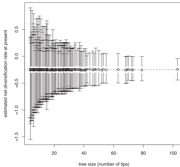
Fig. 54. Confidence intervals around the estimated net diversification rate at present as a function of tree size (number of tips). Each data point and error bar corresponds for a single phylogeny to the estimated net diversification rate at present and 95% confidence interval around it, respectively. Results for the 186 phylogenies with estimated net diversification rates at present falling within -0.26 and -0.24 .
