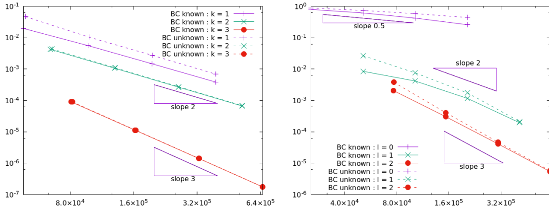
Figure 1: L^2(T_1, T_2; H^1(B)) -seminorm errors with respect to the number of dofs for the 1d test case without any noise. Both cases with known or unknown boundary data are considered. Left: space convergence ( M \in \{16, 32, 64, 128\} , N = 128 , \ell = 3 ). Right: time convergence ( N \in \{10, 20, 40, 80\} , M = 256 , k = 3 ).
