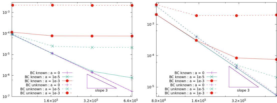
Figure 2: L^2(T_1, T_2; H^1(B)) -seminorm errors with respect to the number of dofs for the 1d test case and various noise levels. Left: space convergence ( M \in \{16, 32, 64, 128\} , k = 3 , N = 128 , \ell = 3 ). Right: time convergence ( N \in \{10, 20, 40, 80\} , \ell = 2 , M = 256 , k = 3 ).
