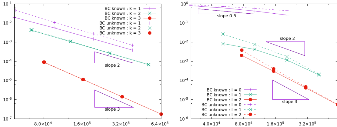
Figure 1: L^2(T_1, T_2; H^1(B)) -seminorm errors with respect to the number of dofs for the 1d test case without any noise. Both cases with known or unknown boundary data are considered. Left: space convergence ( M \in \{16, 32, 64, 128\} , N = 128 , \ell = 3 ). Right: time convergence ( N \in \{10, 20, 40, 80\} , M = 256 , k = 3 ).
