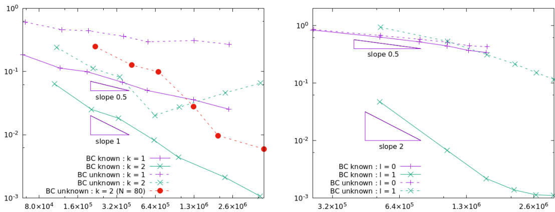
Figure 4: L^2(T_1, T_2; H^1(B)) -seminorm errors for the 2d test case without any noise. Left: space convergence ( N = 40 except the curve with red bullets for which N = 80 , \ell = 1 ). Right: time convergence (finest mesh, k = 2 ).
