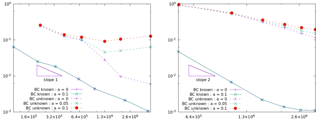
Figure 5: L^2(T_1, T_2; H^1(B)) -seminorm errors for the 2d test case with noised data ( a \in \{0, 0.05, 0.1\} ). Left: space convergence ( k = 2 and \ell = 1 ). Right: time convergence (finest mesh from Figure 3, k = 2 and \ell = 1 ).
