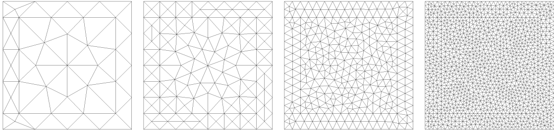
Figure 3: First, third, fifth, and seventh triangulations used for the 2d test case; all the triangulations are fitted to \varpi and B .
