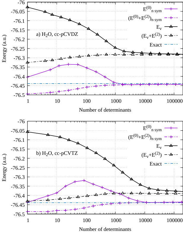
FIG. 3. H 2 O. Convergence of the zeroth order energy and the corrected energy using the selection criterion E_n^{(0)} and comparison with the usual Hermitian CIPSI algorithm in the same basis in the cc-pCVDZ (a) and cc-pCVTZ (b) basis sets. The estimated exact energy is taken from the extrapolated DMC energy of Caffarel et. al. (see Ref. 88).
