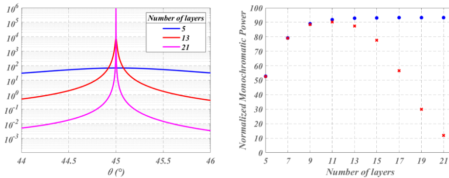
Fig. 16. Angular pattern of the transparent ZAL cavity (left figure) for 3 different layer numbers. The right figure is for the same pattern integrated in the angular range 44^\circ < \theta < 46^\circ and plotted versus the layer number, for a transparent cavity (blue dots) and for imaginary indices of 10^{-5} (red crosses). Data are normalized in regard to the thin layer cavity of Fig. 6 (see text).
