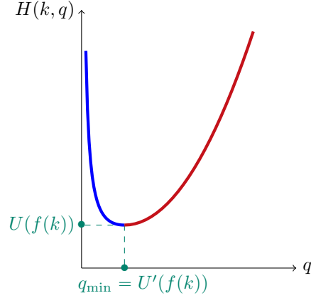
FIGURE 3.1. The bold line (blue and red) is the graph of the function H(k, \cdot) . The blue line is the graph of H^\downarrow(k, \cdot) . The red line is the graph of H^\uparrow(k, \cdot) . In the present figure, \lim_{q \rightarrow 0^+} H(k, q) = +\infty , but it is also possible that \lim_{q \rightarrow 0^+} H(k, q) \in \mathbb{R} .
