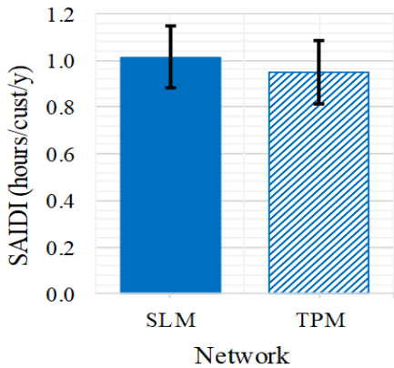
(a) SAIDI
