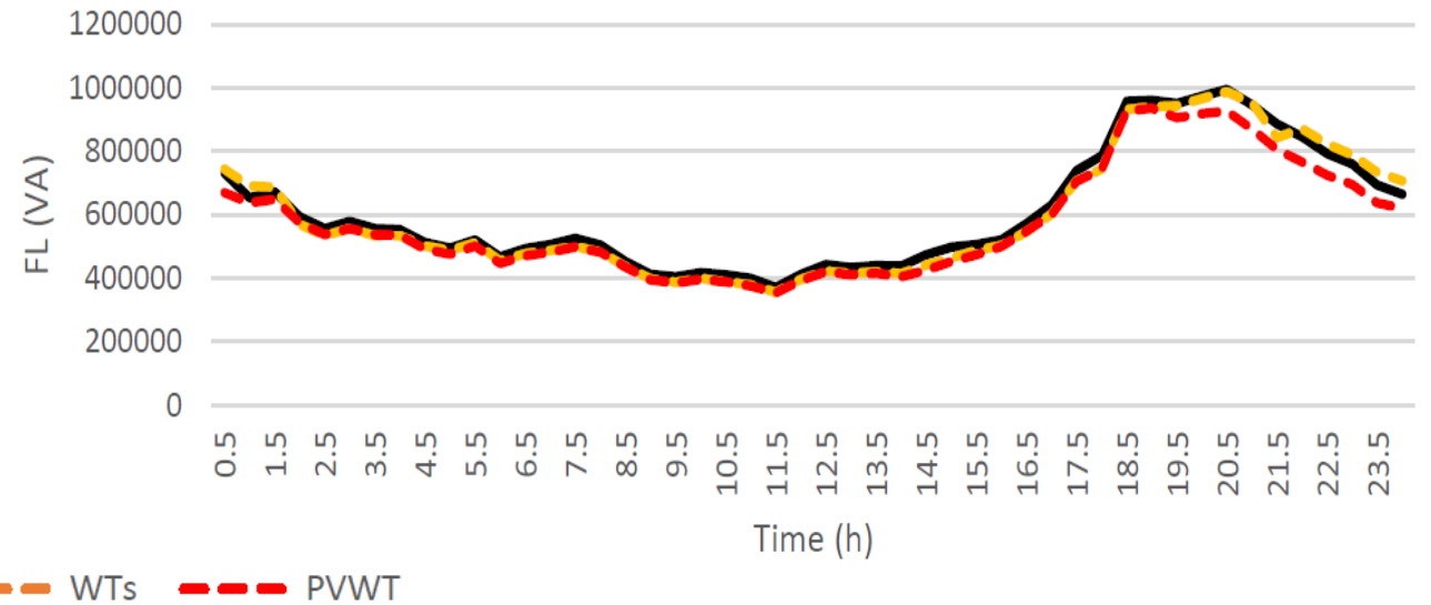
Steady-state Fault Level at LV Transformer (0,4kV)
