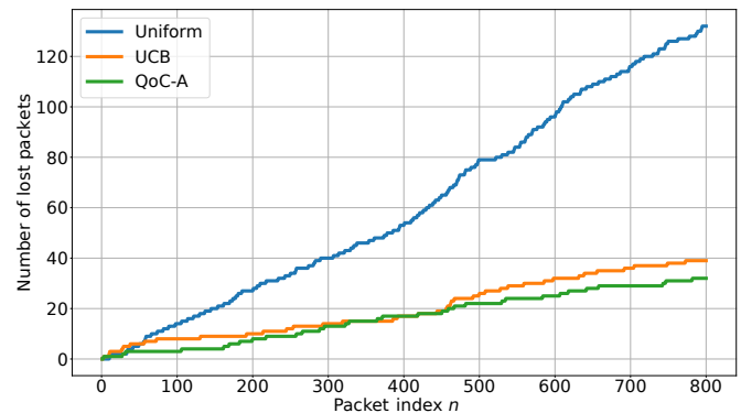
(b) Cumulative regret over 800 steps.
