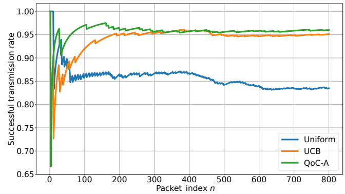
(a) Average reward over 800 steps.
