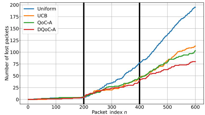
(b) Cumulative regret over 600 steps.
