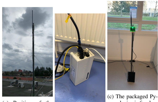
(a) Position of the gateway monopole antenna fixed on the roof of the IETR lab. (b) The gateway connected to the antenna to a battery inside a building. (c) The packaged Pycom device is fixed on a rod and connected to a battery inside a building.
