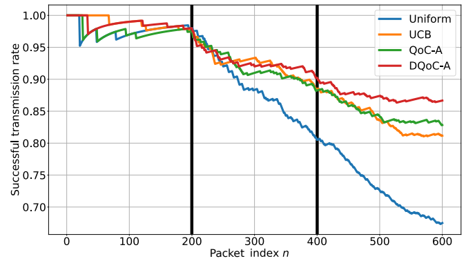
(a) Average reward over 600 steps.
