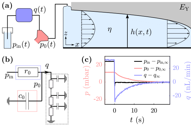
Figure 1. (a) Schematics of the microfluidic setup, including a flow sensor, a pressure sensor and a soft channel. (b) Equivalent electronic circuit, the flow sensor modeled as an ideal resistance r_0 , the pressure sensor as a capacitance c_0 , and the soft channel as a series of infinitesimal resistances and capacitances as in a transmission line. (c) Shifted, imposed p_{in} and measured p_0 and q as a function of t , with long-time values of p_{in,\infty} = 1301 mbar, p_{0,\infty} = 862 mbar and q_\infty = 1058 nL/min.
