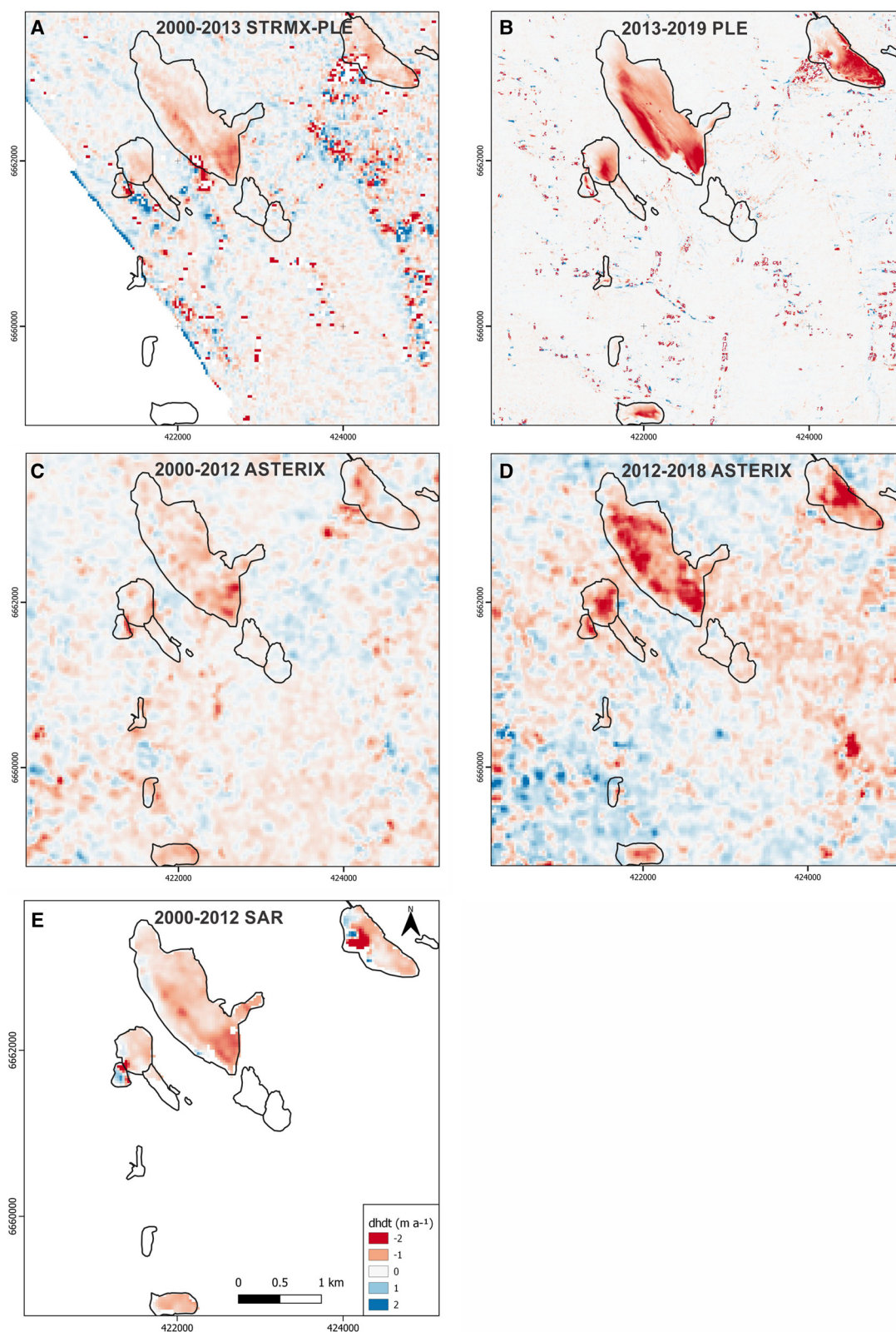
Fig. 6. Maps of annual elevation change rate ( dh/dt ) at Agua Negra glacier and nearby ice masses. (a) SRTMX 2000–PLÉ 2013 DEM differences, (b) PLÉ–2013–2019, (c) ASTERIX 2000–2012, (d) ASTERIX 2012–2018 and (e) SAR 2000–2012. The glacier outlines are from the year 2000 and the maps have the same color code for dh/dt to highlight the increase in downwasting rates in the more recent periods.
