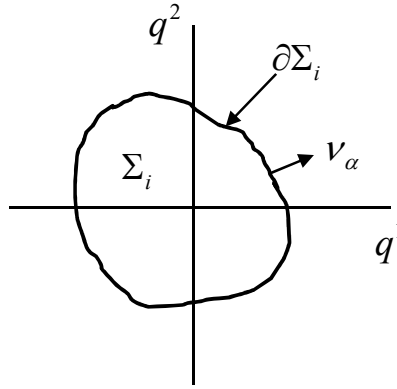
Figure 3: The equilibrium interface, \Sigma_i , and contact line, \partial\Sigma_i , in the q^\alpha plane. v_\alpha is normal to \partial\Sigma_i .
