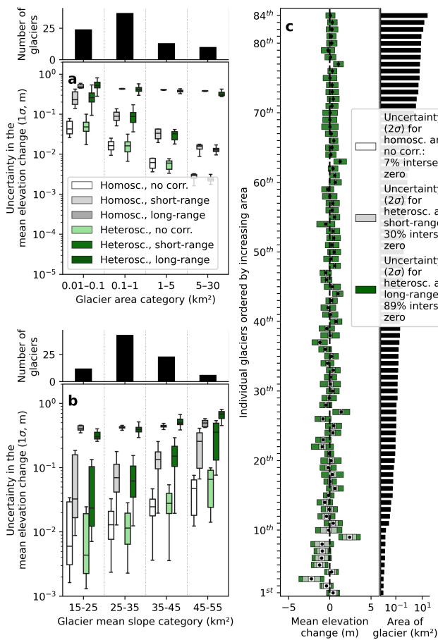
Fig. 7. Uncertainty propagation to glacier mean elevation changes at the Mont-Blanc massif. a-b, Distributions of uncertainty of glacier mean elevation change by category of area and average terrain slope for each set of assumption, with boxes denoting the interquartile range and whiskers extending to the entire distribution. c, Empirical evaluation of uncertainty ranges for mean glacier elevation changes in the Mont-Blanc case study. Correct uncertainty estimates should cross the vertical zero line in 95% of the cases.
