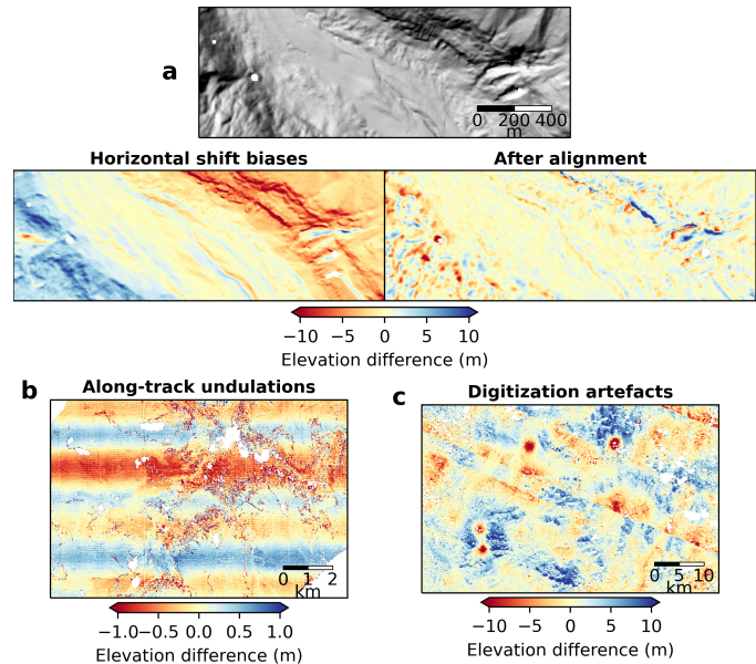
Fig. 1. Patterns of random and systematic errors in DEMs. a, Elevation differences of horizontal shifts (left) and after alignment (right) with terrain hillshade (top), extracted from the data in Table I. The horizontal shift between Pléiades and SPOT-6 DEMs is of 2 m east and 4 m north, creating large biases despite being relatively small (half a pixel). b-c, Noise owed to (b) along-track undulations in a Pléiades–Pléiades DEM difference and to (c) digitization artefacts in a KH-9–ArcticDEM DEM difference [13], after alignment.
