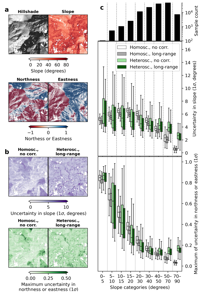
Fig. 6. Uncertainty propagation to terrain slope and aspect at the Mont-Blanc summit. a, Hillshade and terrain attributes based on the Pléiades DEM. b, Slope and aspect uncertainty estimated by the half-difference between the 16 th and 84 th percentiles of 1,000 simulated terrain attributes at each pixel. c, Distributions of slope and aspect uncertainties by category of terrain slope for each set of assumptions, with boxes denoting the interquartile range and whiskers extending to the entire distribution.
