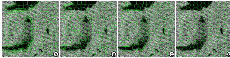
Fig. 4: Tested super-pixels for SHAP method, delimited in green. One compares automatic clustering approaches (A-C) and a predefined hexagonal grid (D).
