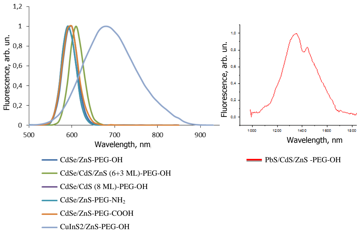
Figure S2. Fluorescence spectra of quantum dots modified with polyethylene glycol derivatives.
