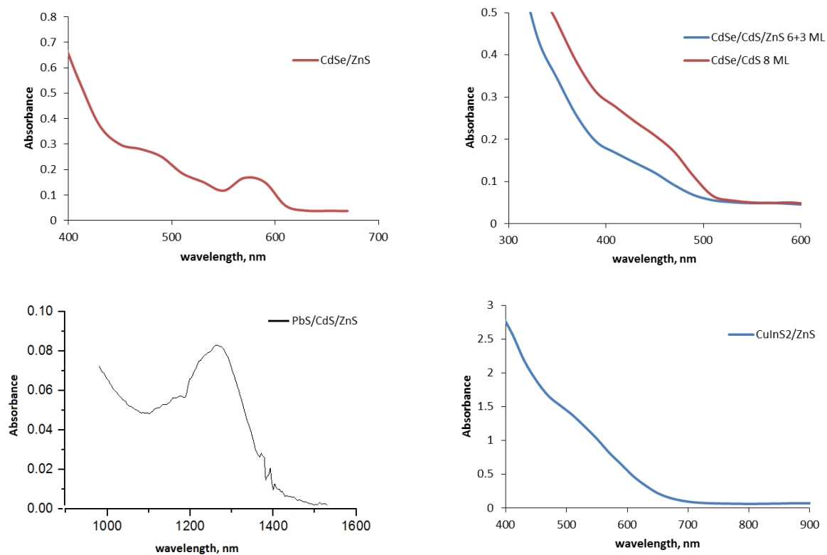
Figure S1. Absorption spectra of the as-synthesized water-insoluble quantum dots.
