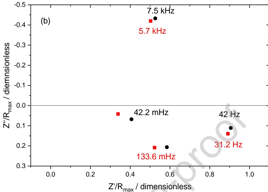
Fig. 4. Nyquist plots of the impedance response at two different rotation rates ( \Omega = 500 rpm (black circles) and \Omega = 1000 rpm (red squares)) of Mg after 30 min at E_{\text{corr}} in 1 M \text{Na}_2\text{SO}_4 (pH = 1.8): (a) raw impedance diagrams; (b) normalized impedance diagrams (normalized by R_{\text{max}} , the maximum of the real part of each diagram).
