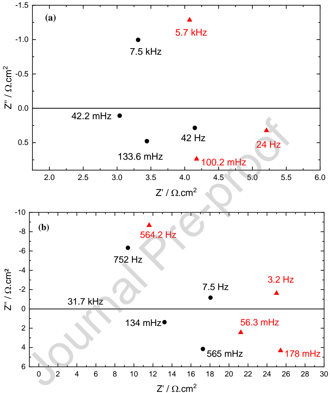
Fig. 2. Electrochemical impedance diagrams of Mg after 30 min (black circles) and 2 h (red triangles) at E_{\text{corr}} and \Omega = 1000 rpm: (a) in 1 M Na 2 SO 4 , pH = 1.8; (b) in 1 M N Na 2 SO 4 , pH = 2.9.
