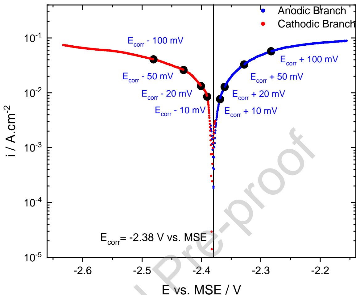
Fig. 5. Current-potential curve of Mg, corrected from the ohmic drop, measured after 30 min at E_{\text{corr}} in 1 M \text{Na}_2\text{SO}_4 acidified at pH = 1.8 ( \Omega = 1000 \text{ rpm} , \nu = 0.1 \text{ mV s}^{-1} ).
