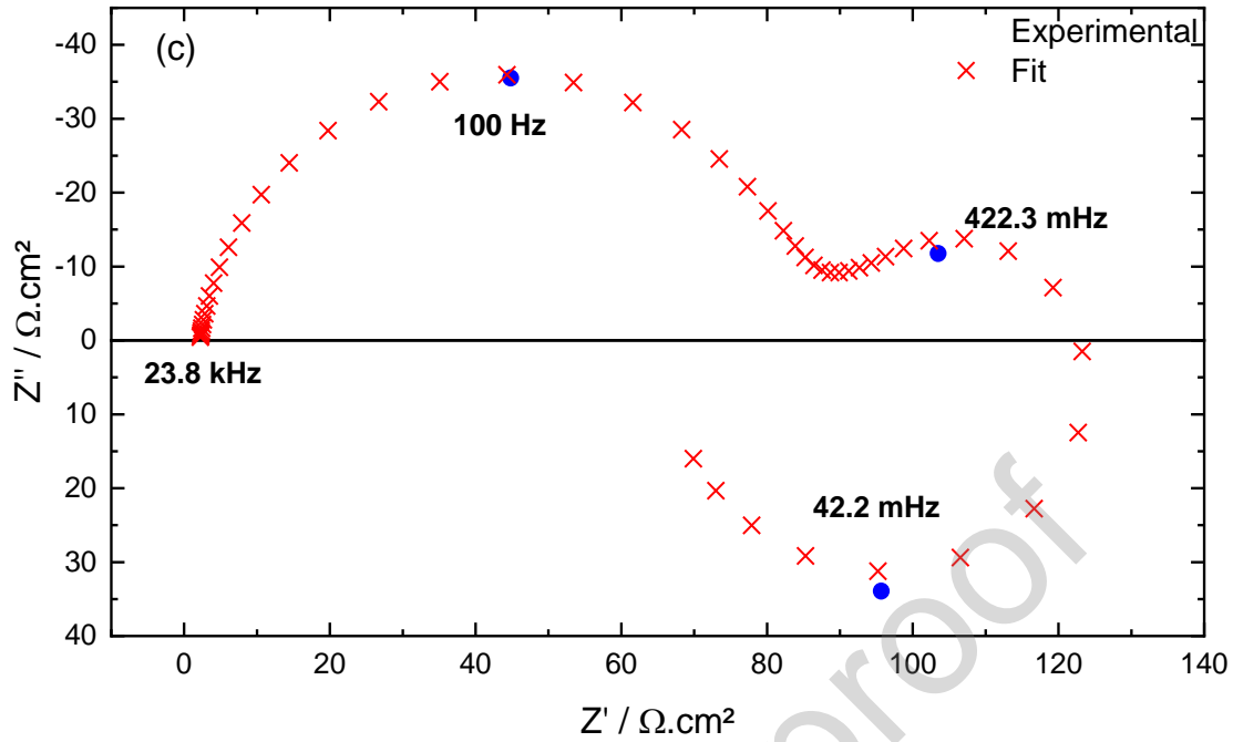
Fig. 8. Impedance diagrams of the Mg electrode after 30 min at E_{\text{corr}} in 1 M \text{Na}_2\text{SO}_4 ( \Omega = 1000 rpm) (blue circles) and the result of the fitting procedure with the model (Eqs. (30) and (33)) (red crosses) at (a) pH = 1.8, (b) pH = 2.9, and (c) pH = 7.7.
