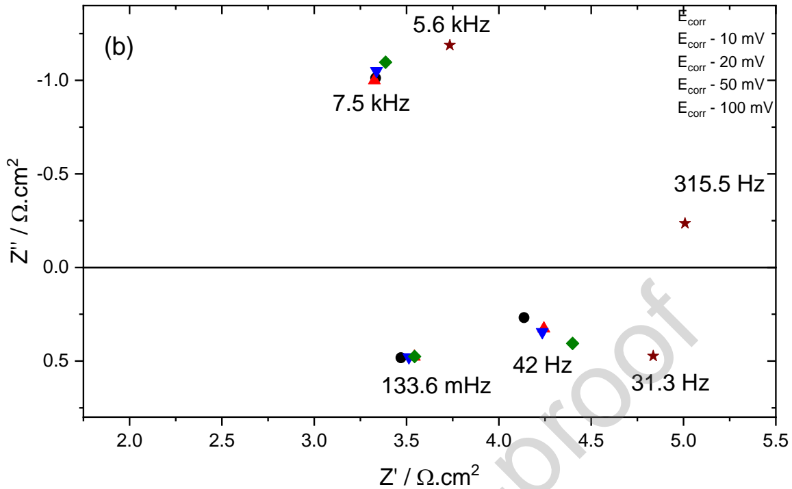
Fig. 6. Electrochemical impedance diagrams of Mg after 30 min at E_{\text{corr}} in 1 M \text{Na}_2\text{SO}_4 acidified at pH = 1.8 ( \Omega = 1000 rpm) at different (a) anodic and (b) cathodic overpotentials.
