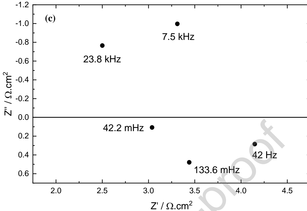
Fig. 1. Electrochemical impedance diagrams (Nyquist representation) of Mg after 30 min immersion at E_{corr} in 1 M \text{Na}_2\text{SO}_4 solution at different pH values (electrode rotation rate \Omega = 1000 rpm): (a) pH = 7.7; (b) pH = 2.9; (c) pH = 1.8.
