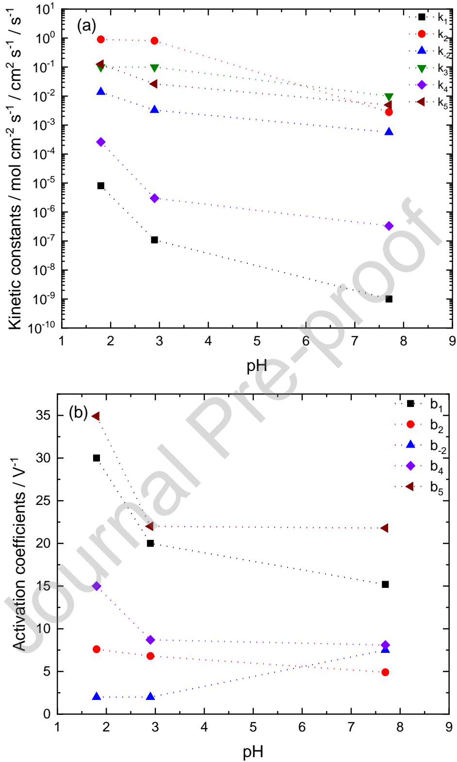
Fig. 9. Variations of the different kinetic parameters related to the corrosion of the Mg electrode after 30 min at E_{\text{corr}} in 1 M Na 2 SO 4 ( \Omega = 1000 rpm) as function of the pH: (a) kinetic constants and (b) activation coefficients.
