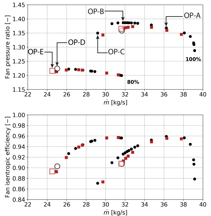
FIGURE 4. MASS-AVERAGED FAN CHARACTERISTICS AT 80% AND 100% OF THE DESIGN SPEED FROM STEADY AND UNSTEADY SIMULATIONS: TOTAL PRESSURE RATIO AND ISENTROPIC EFFICIENCY.
