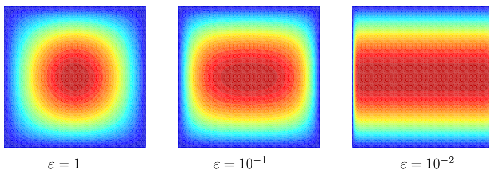
Figure 8: Reaction-diffusion problem with a boundary layer solution: isovalues of u_\varepsilon .
