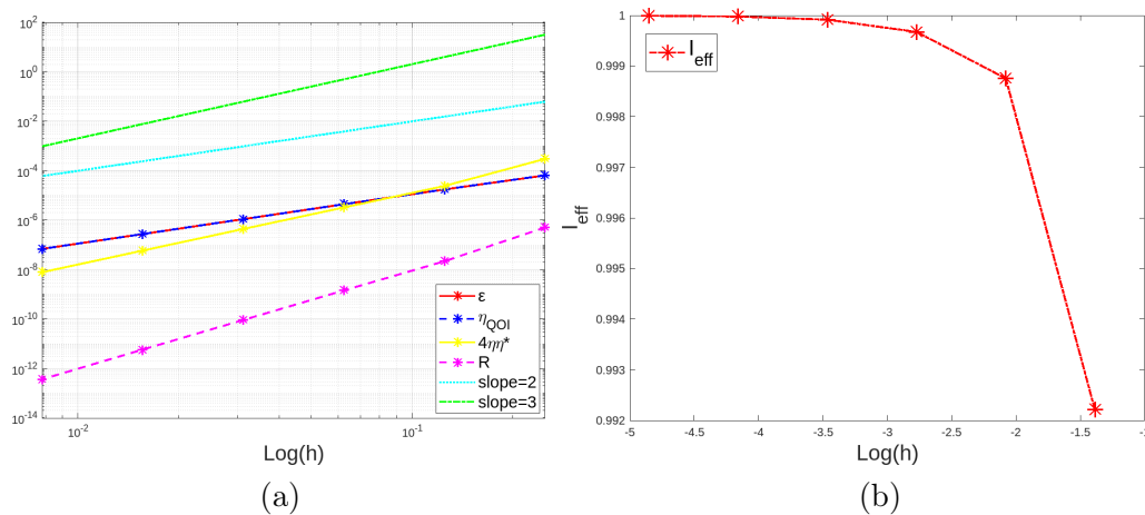
Figure 9: A boundary layer problem, \varepsilon = 1 : (a) rates of convergence; (b) effectivity index I_{eff} .
